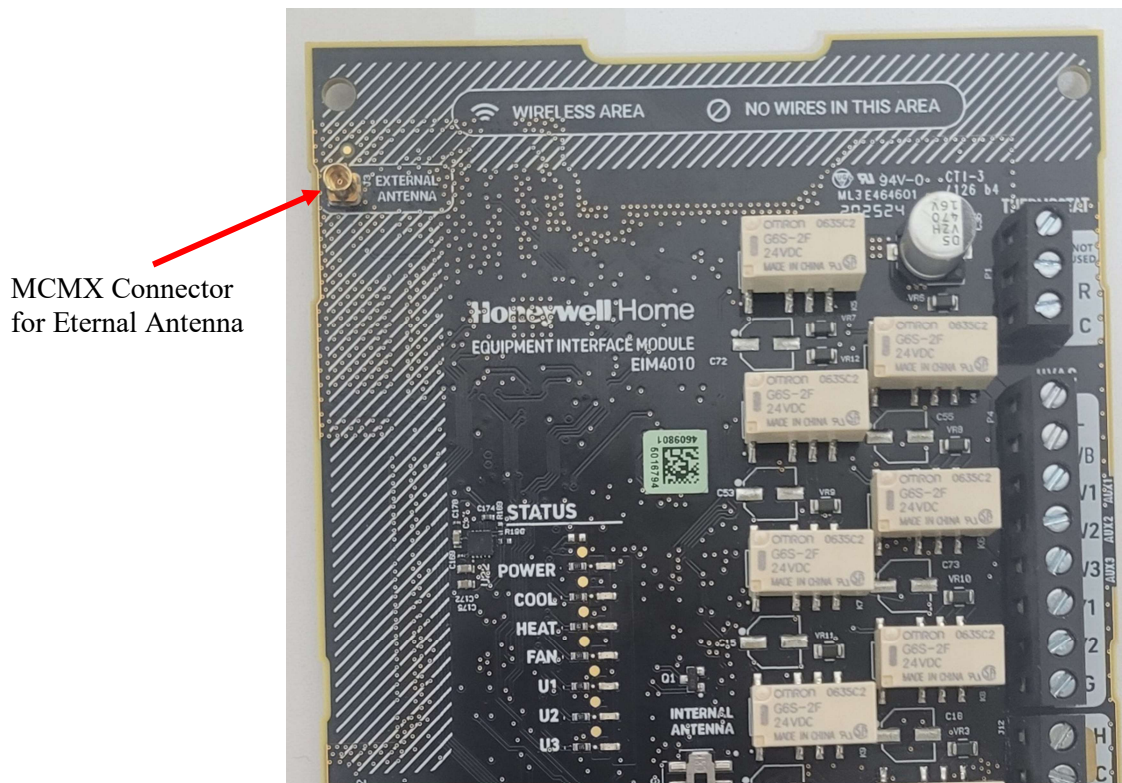
Figure 5 - MCMX connector used to install optional external antenna
