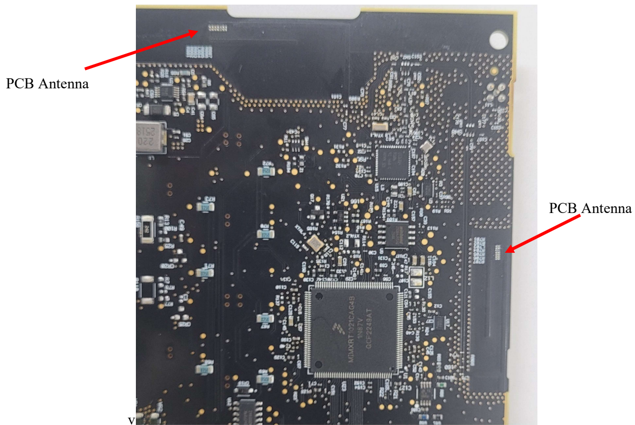
Figure 4 – location of 2 PCB antennas
