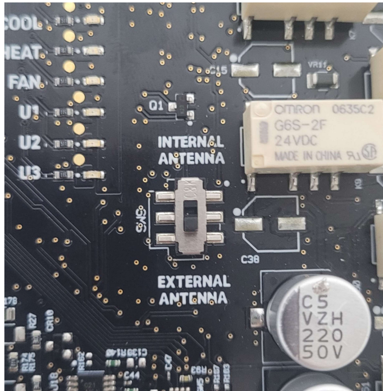
Figure 6 – Switch to select between internal antenna or external antenna
