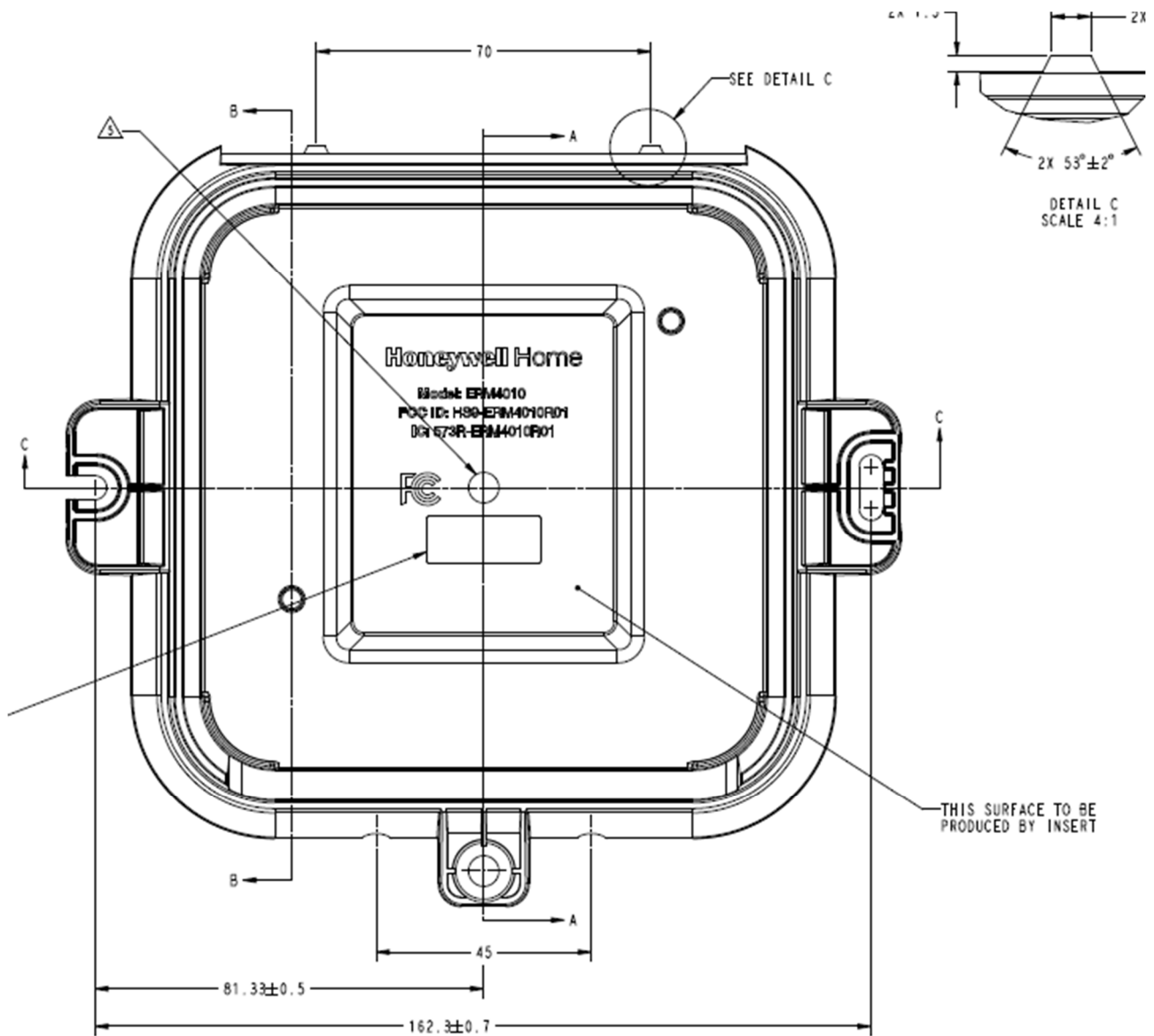
Figure 1 – Label Location etched on device back side
