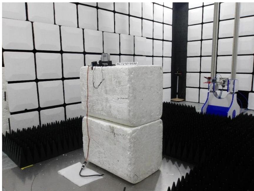
Photo 1-10 – Radiated Spurious Emissions 1GHz – 18GHz – Rear View
