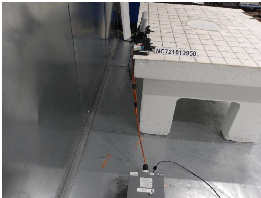
Photo 2-2 – Power Line Conducted Emissions – Side View
