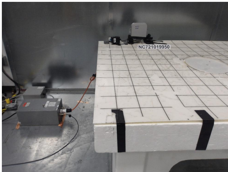
Photo 2-1 – Power Line Conducted Emissions – Front View
