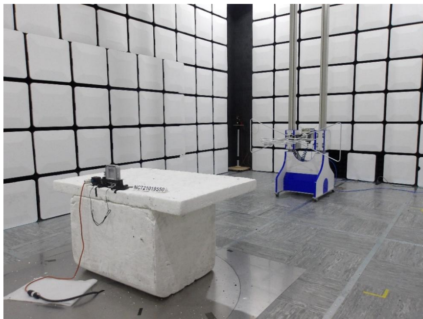
Photo 1-8 – Radiated Spurious Emissions 30MHz – 1GHz – Rear View
