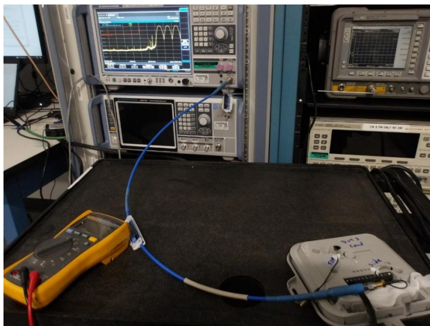
Photo 3-1 – RF Conducted Measurements
