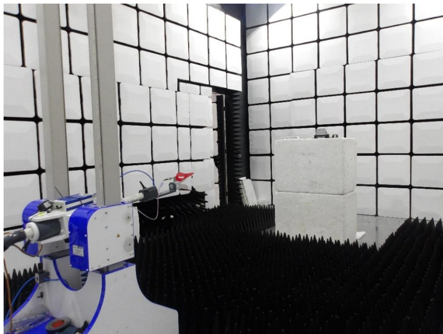
Photo 1-9 – Radiated Spurious Emissions 1GHz – 18GHz – Front View
