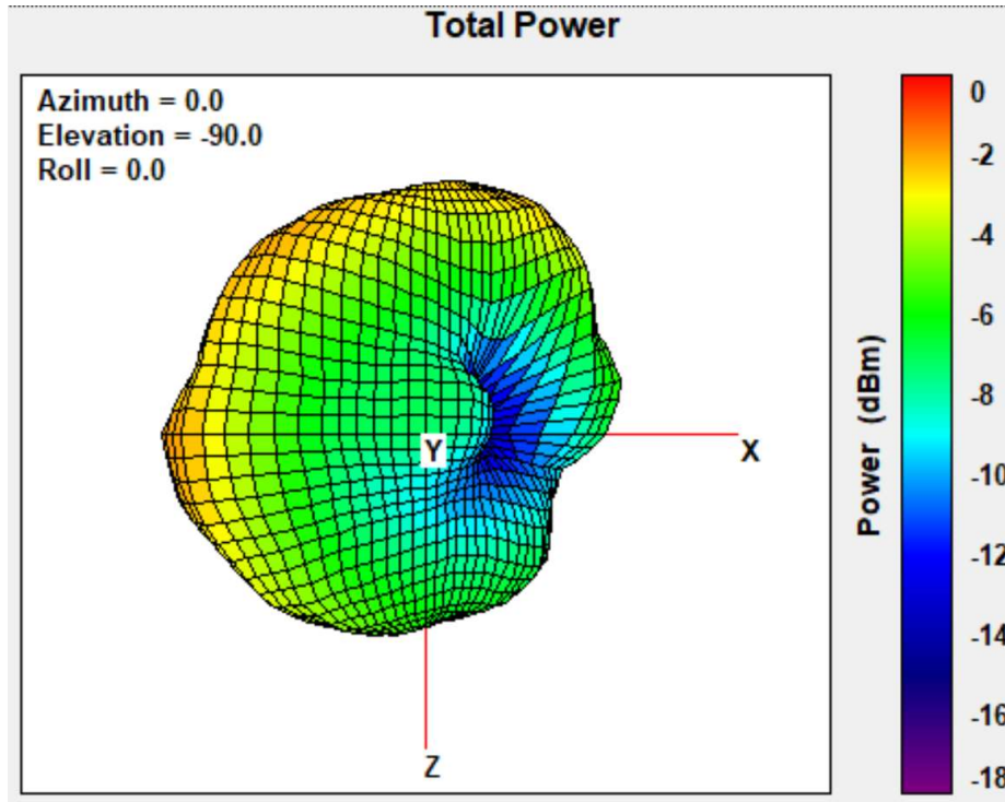
Figure 3. DiagnostIQ Indoor Sensor Hub Antenna 903 MHz Top View
