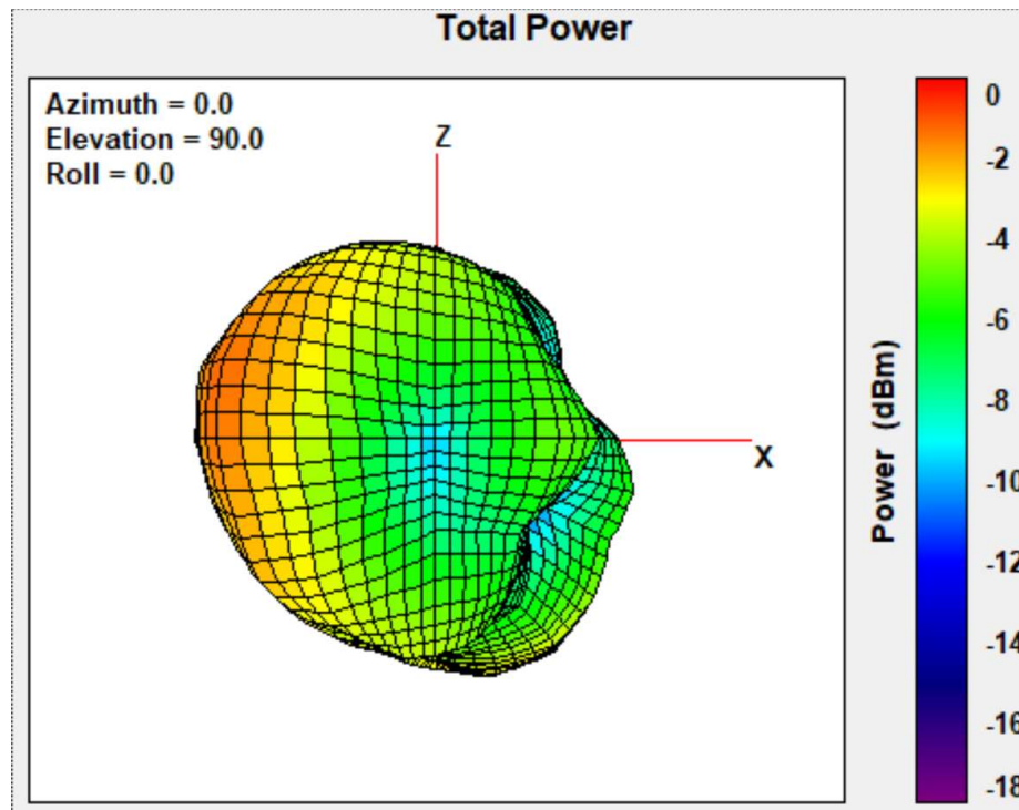
Figure 4 DiagnostIQ Indoor Sensor Hub Antenna 903 MHz Bottom View
