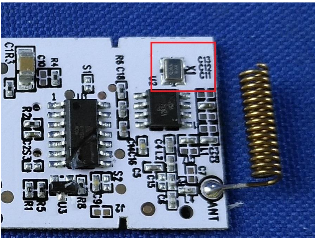
Oscillator Location
