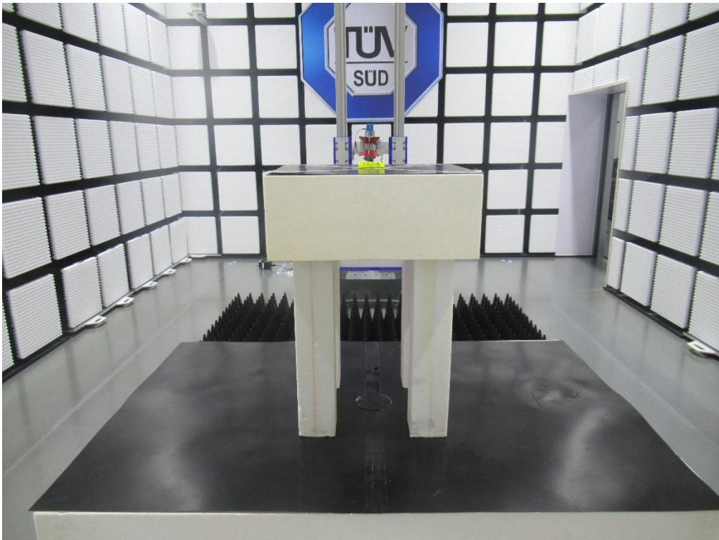
Radiated Emissions Test above 1GHz
