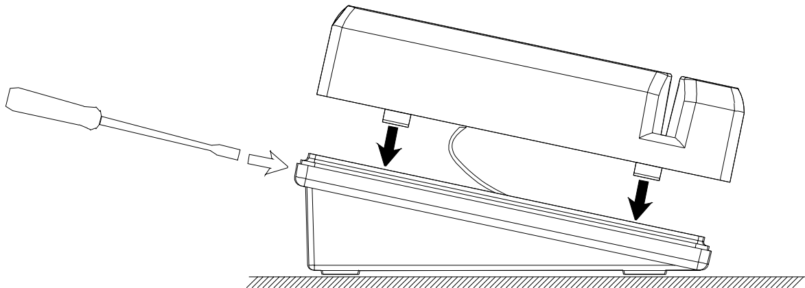
Figure 12: Closing the terminal (anchor-mounted assembly)
