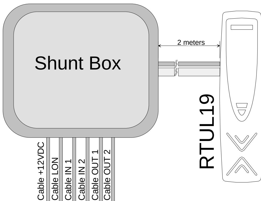
Figure 3: Shunt Box
