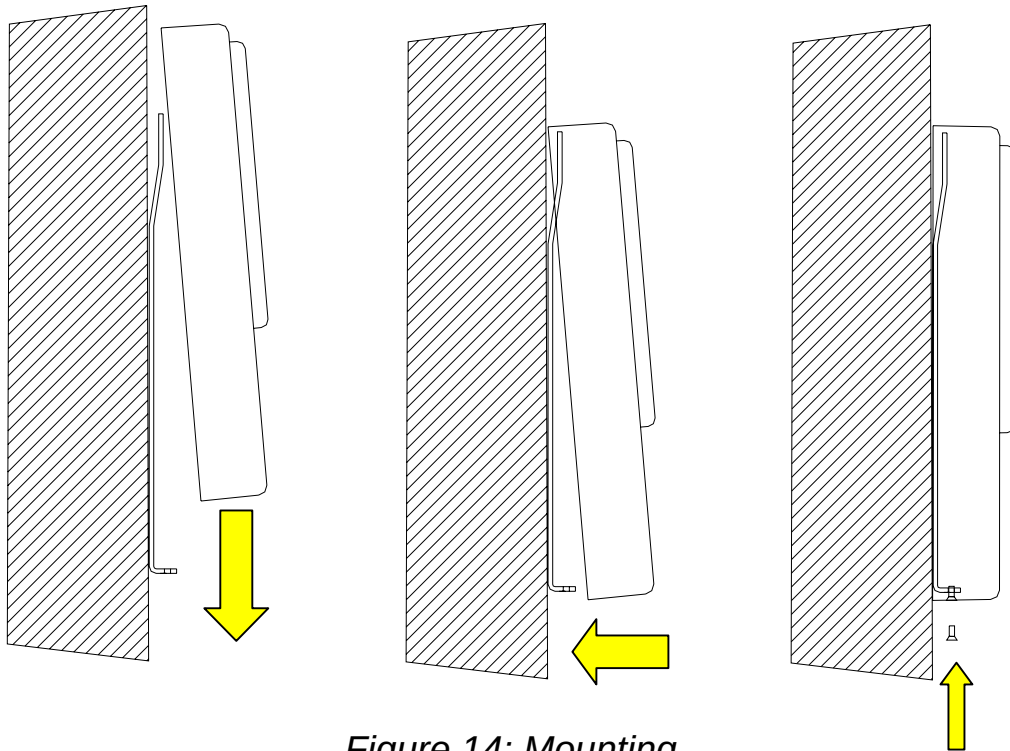
Figure 14: Mounting
