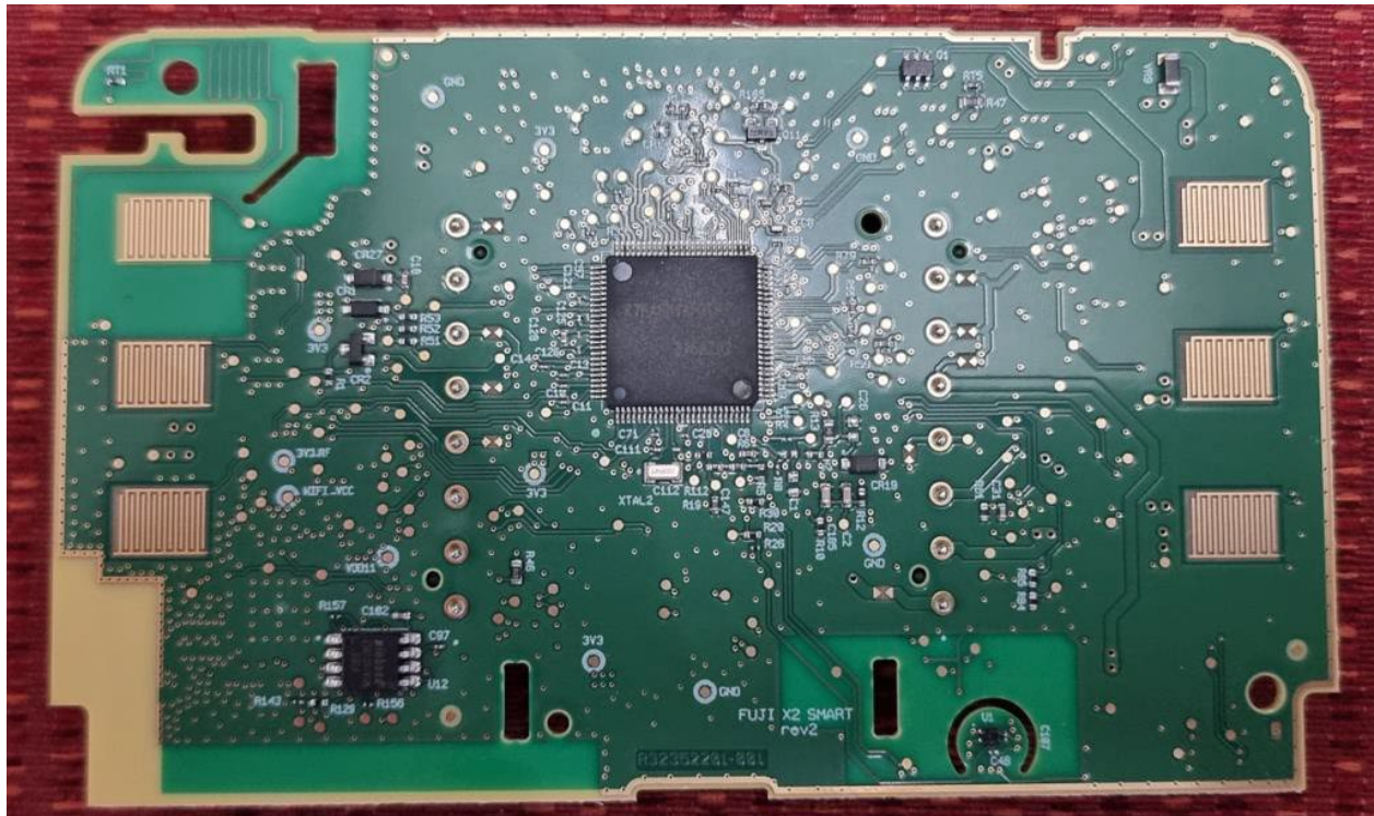
Figure 16 PCB front view without display
