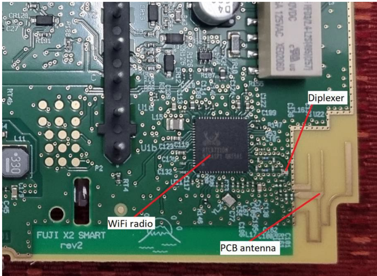
Figure 15 Wi-Fi Radio
