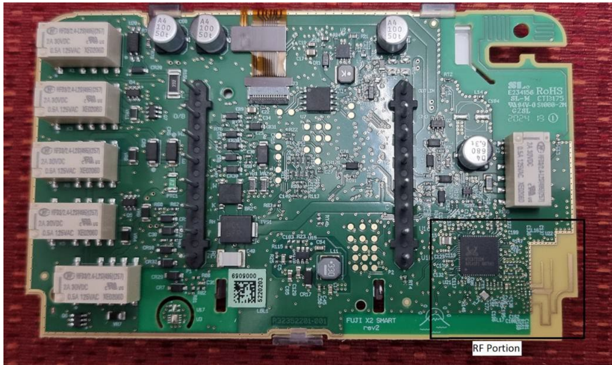
Figure 10 Back side view
