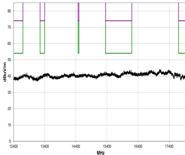
12400-18000 MHz, Run 86
