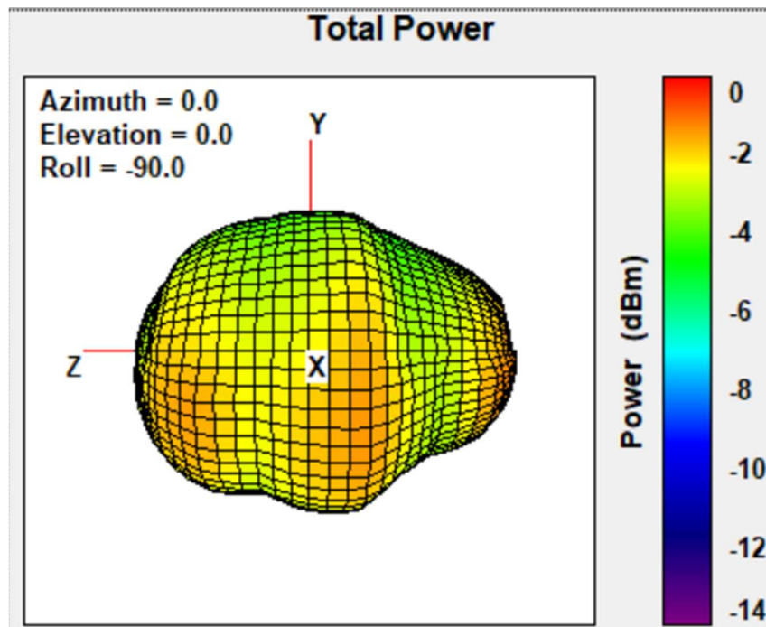
Figure 6. TH6320ZW2007S2 908.4 MHz Right Side View
