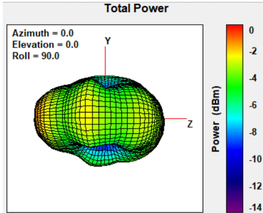
Figure 5. TH6320ZW2007S2 908.4 MHz Left Side View
