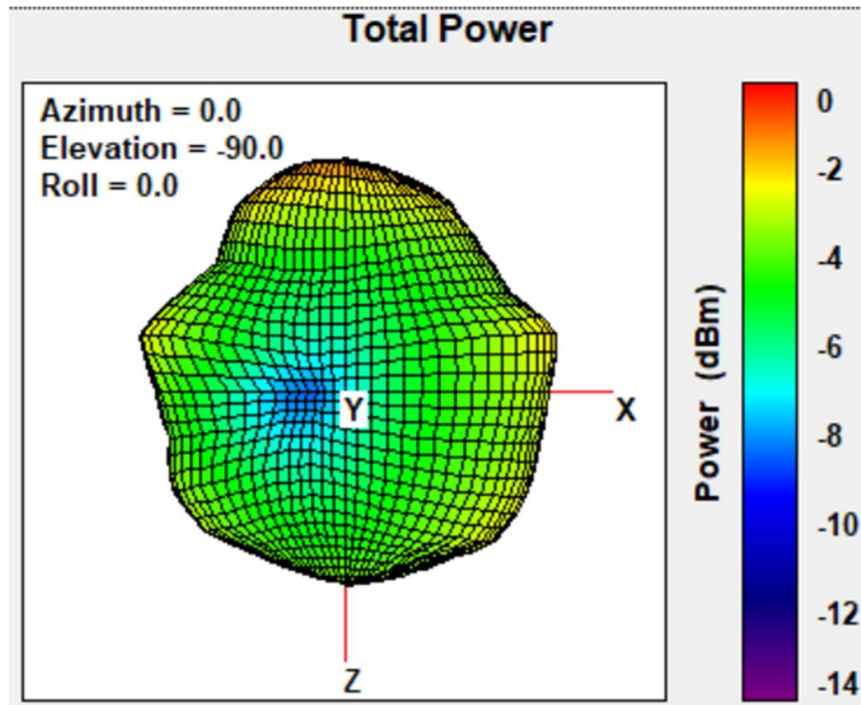
Figure 3. TH6320ZW2007S2 908.4 MHz Top View
