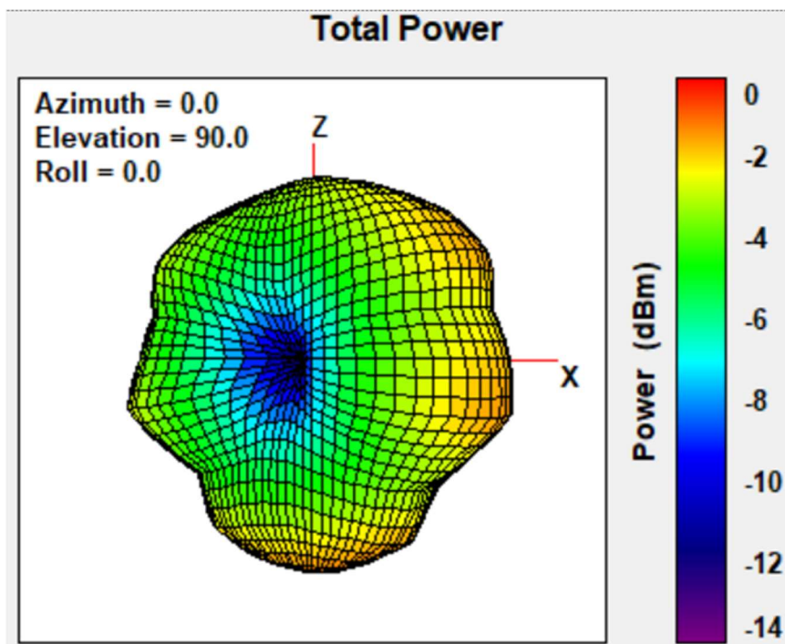
Figure 4 TH6320ZW2007S2 908.4 MHz Bottom View
