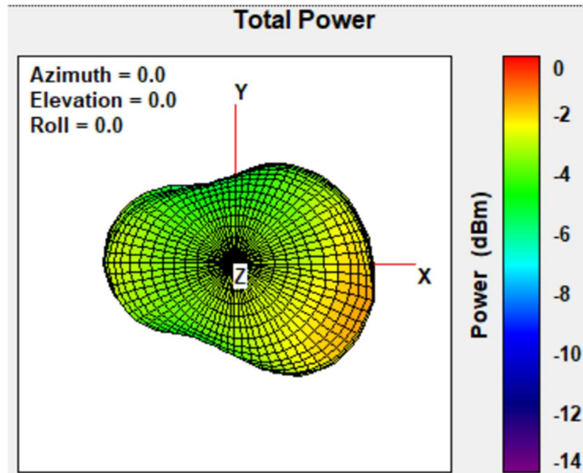
Figure 1. TH6320ZW2007S2 908.4 MHz Front View
