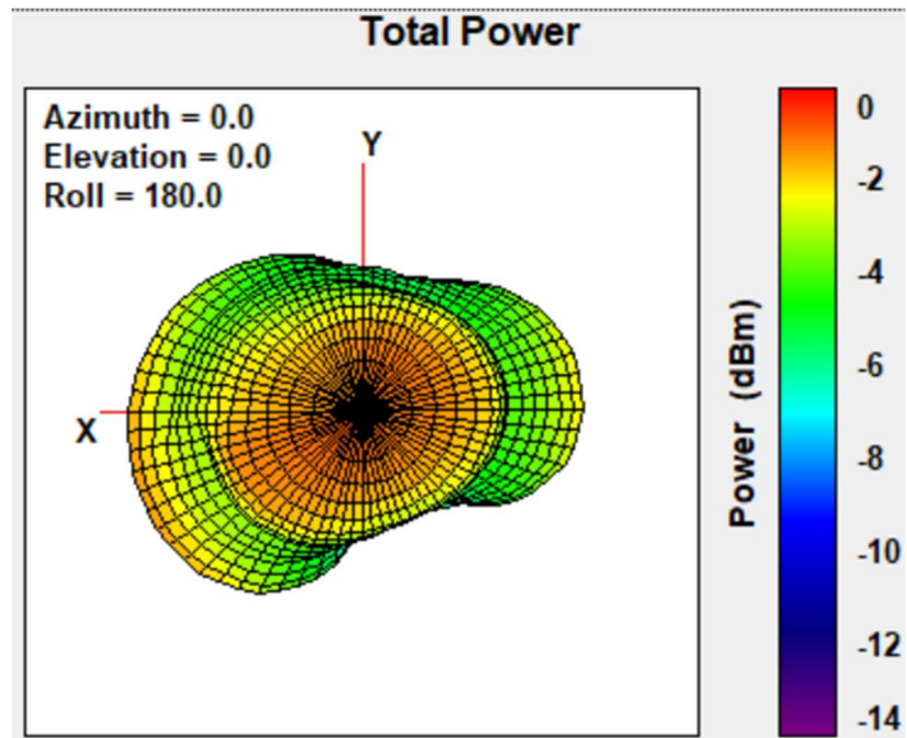
Figure 2. TH6320ZW2007S2 908.4 MHz Back View
