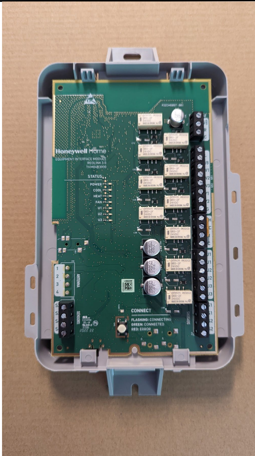
Figure 8. Front side view with cover removed.
