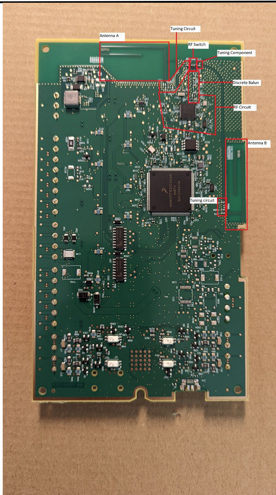
Figure 4. RF circuit identification.
