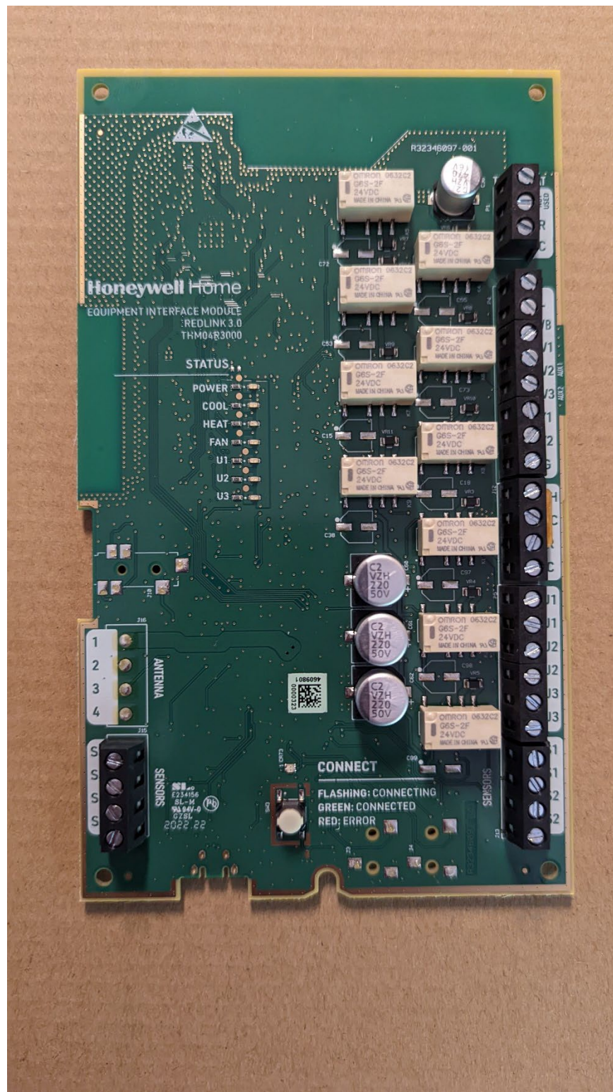
Figure 1. PCB Top side view.
