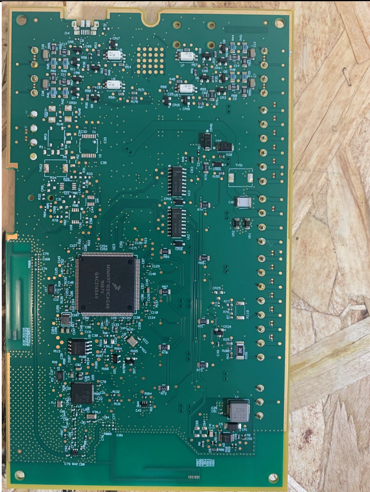
Figure 2. PCB Back side view.
