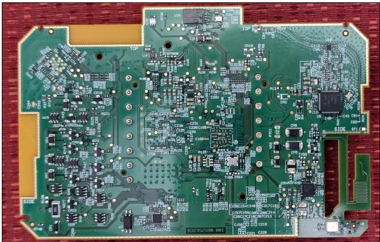
Figure 5. Front side view.
