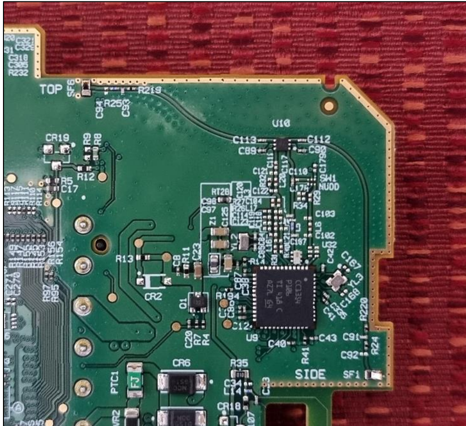
Figure 7. Close view on CC1354P10 radio.
