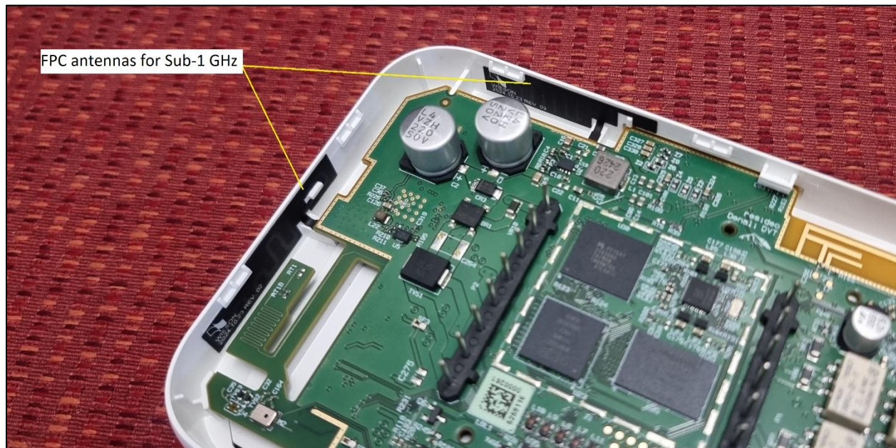
Figure 2. Back side view, focus on Sub-1 GHz FPC antennas.
