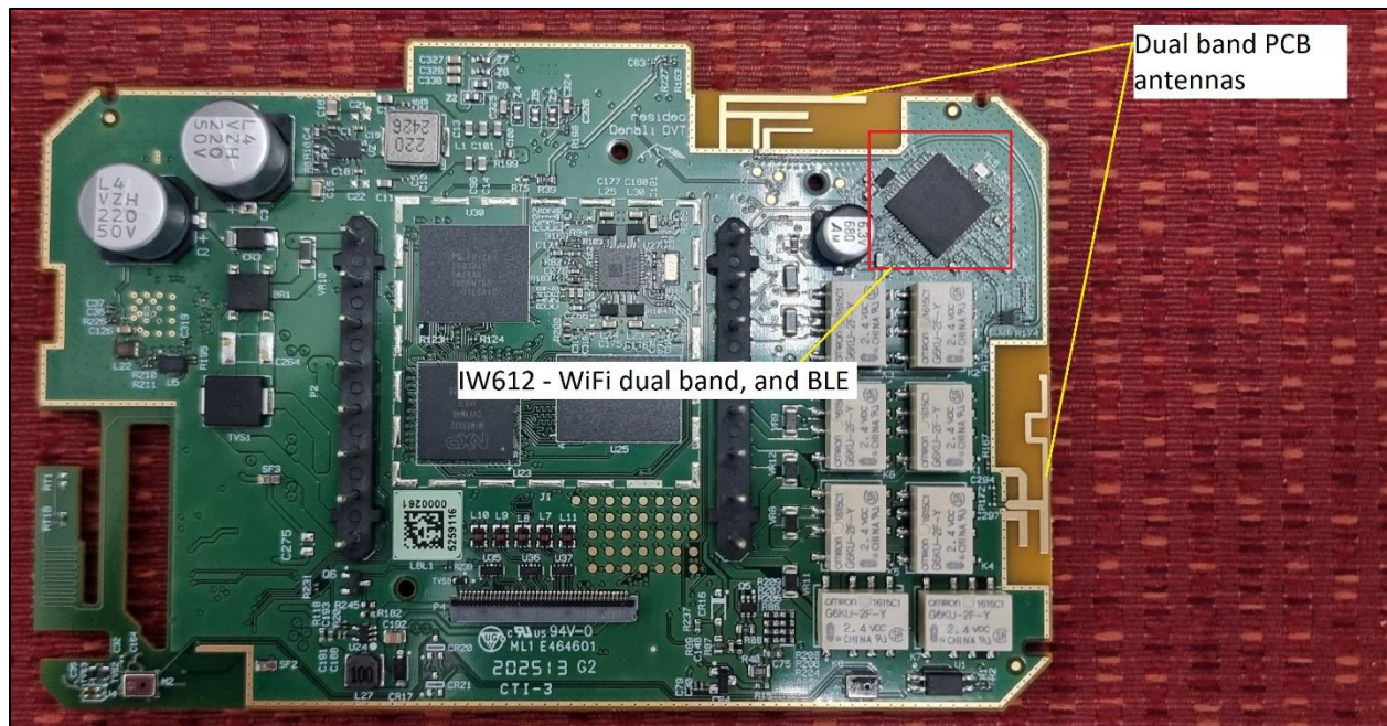
Figure 3. Back view. WiFi & BLE radio.
