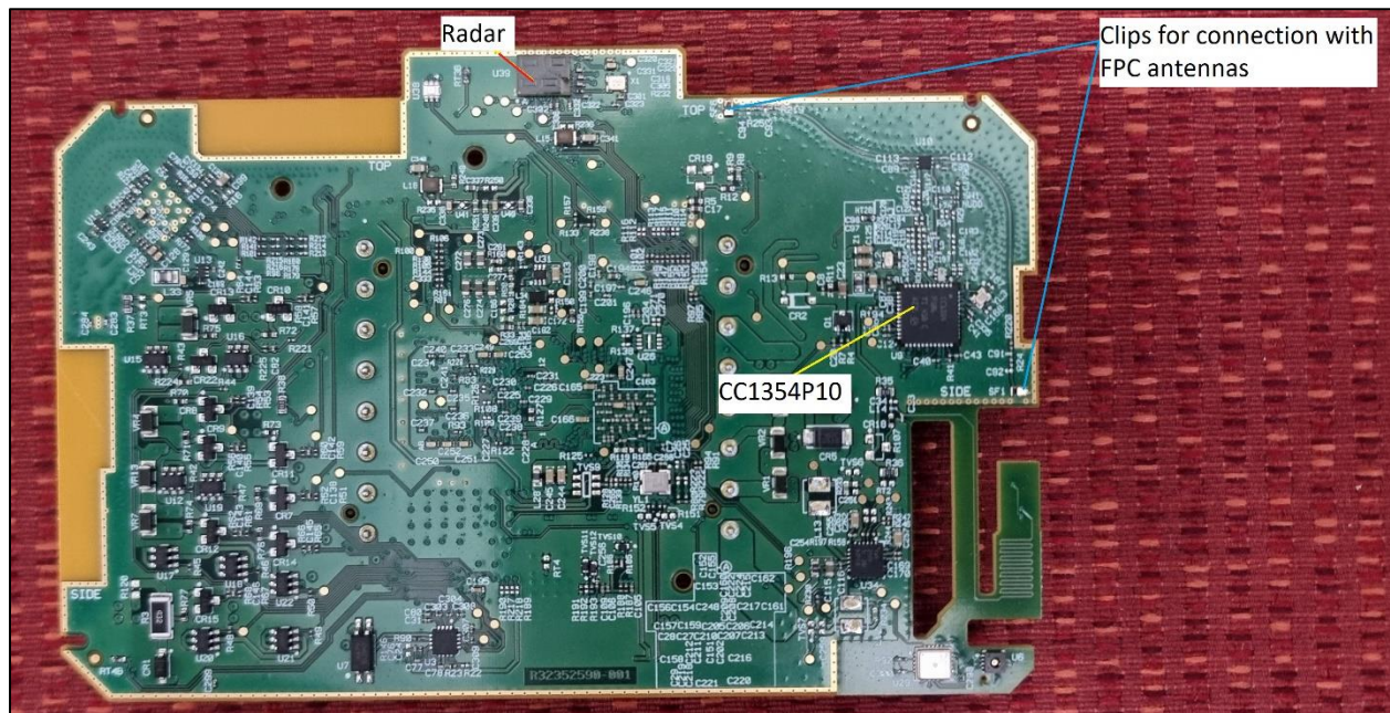
Figure 6. Front side view. Radar and CC1354P10 radio.
