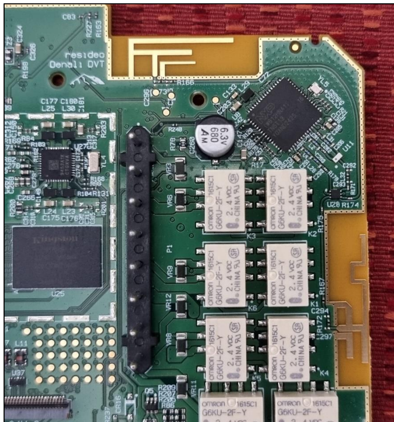
Figure 4. Close view on WiFi & BLE (IW612) radio.
