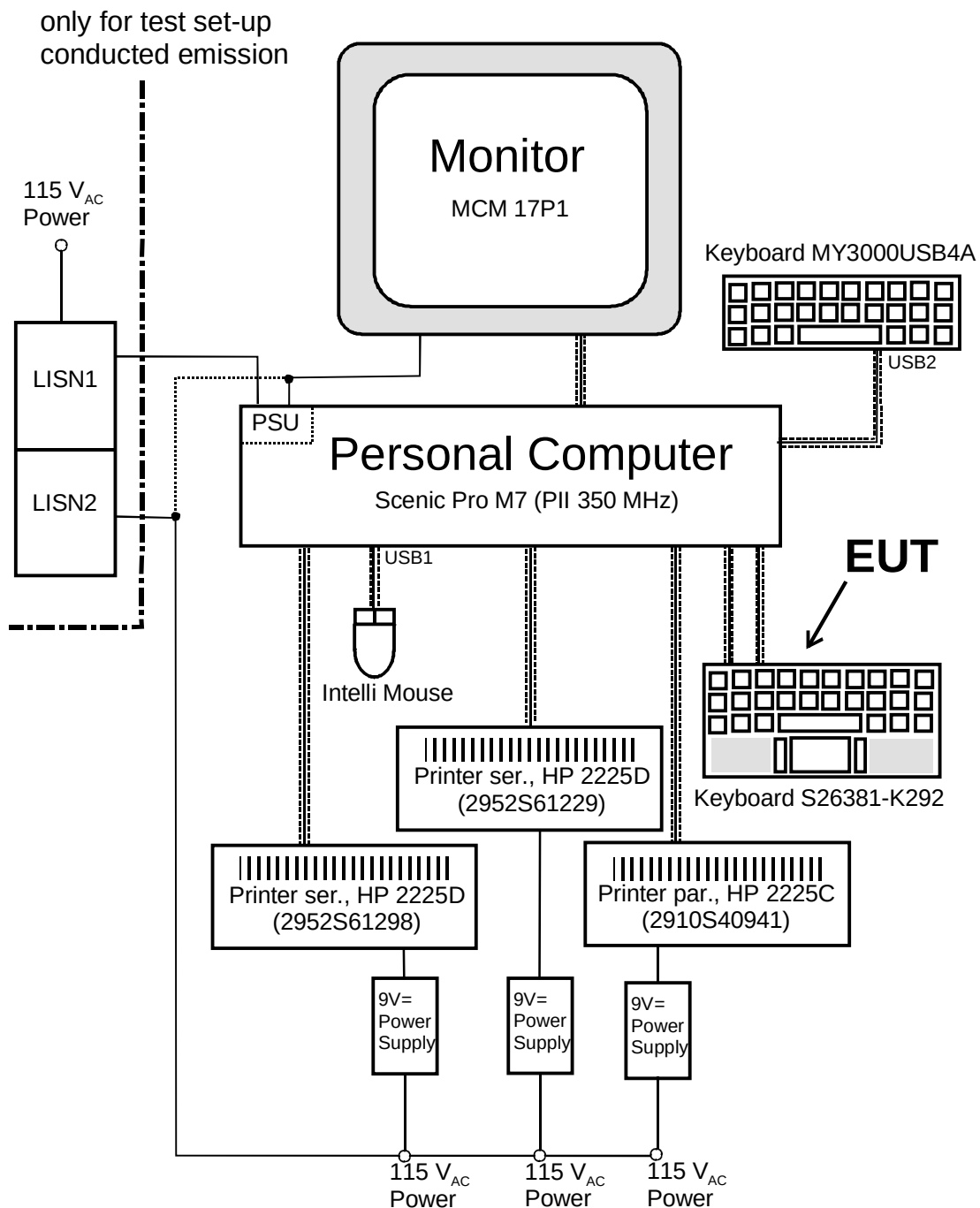
Figure 3.1 Configuration of Tested System
