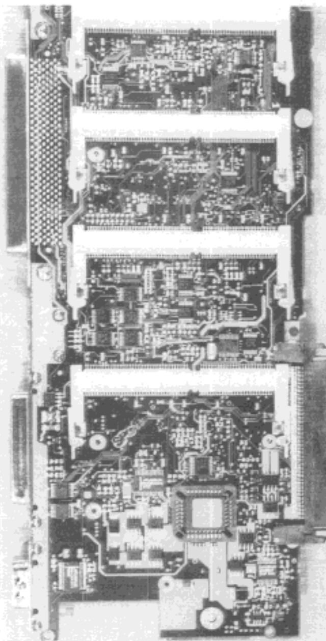
8.23 System board, rear side view, part two
