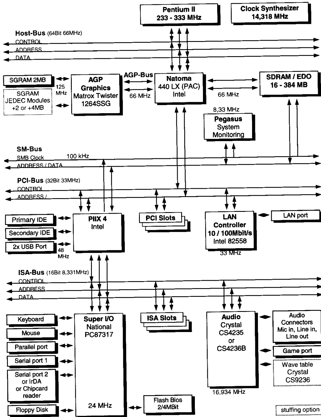
Figure 4.1 Block Diagram of the EUT
