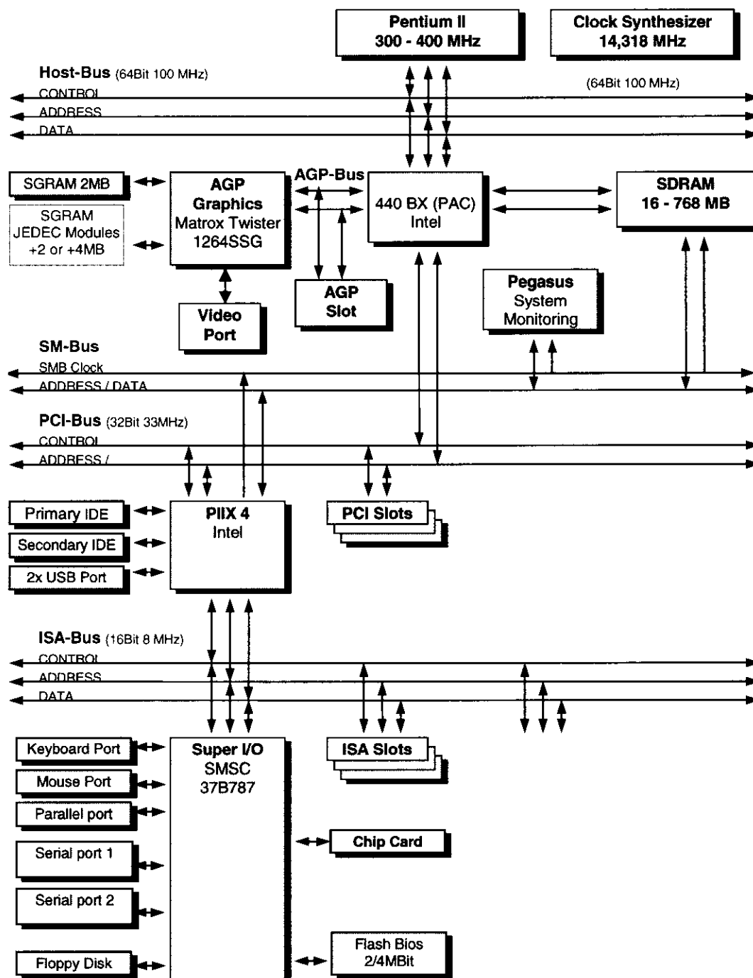
Figure 4.1 Block Diagram of the EUT
