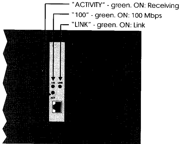
Figure 10. Status LEDs
