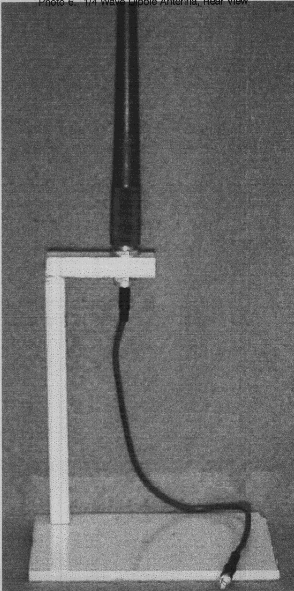
Photo 6. 1/4 Wave Dipole Antenna, Rear View
