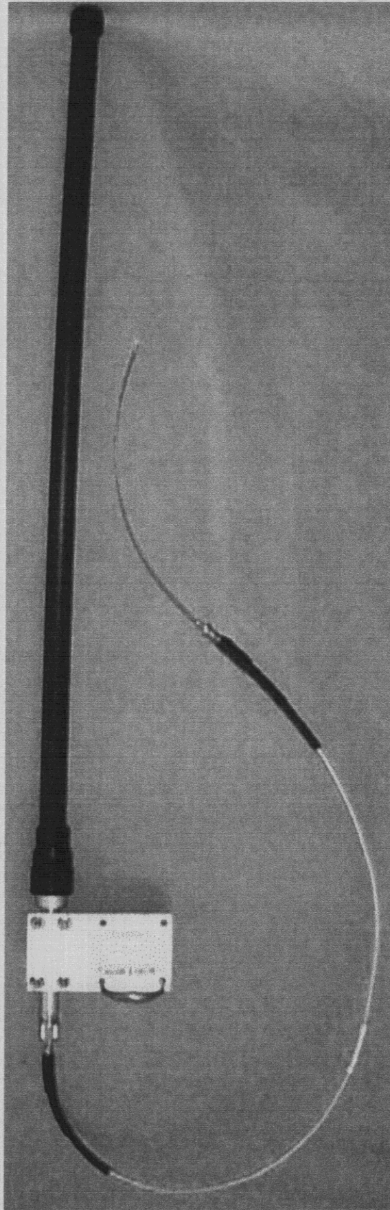
Photo 2. 12 dB Omni Antenna, Rear View
