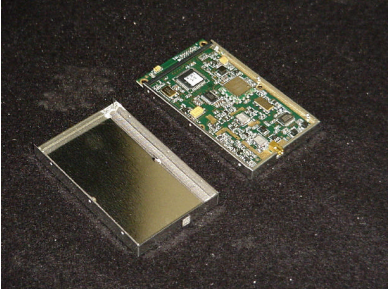
Photo 3. Top of EUT, Cover Open
