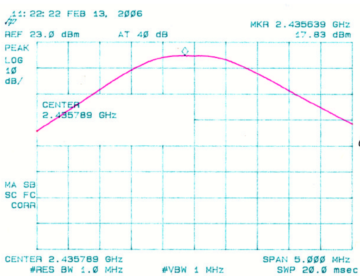
Figure 3b. Peak Power per FCC Section 15.247( b) Mid Channel
