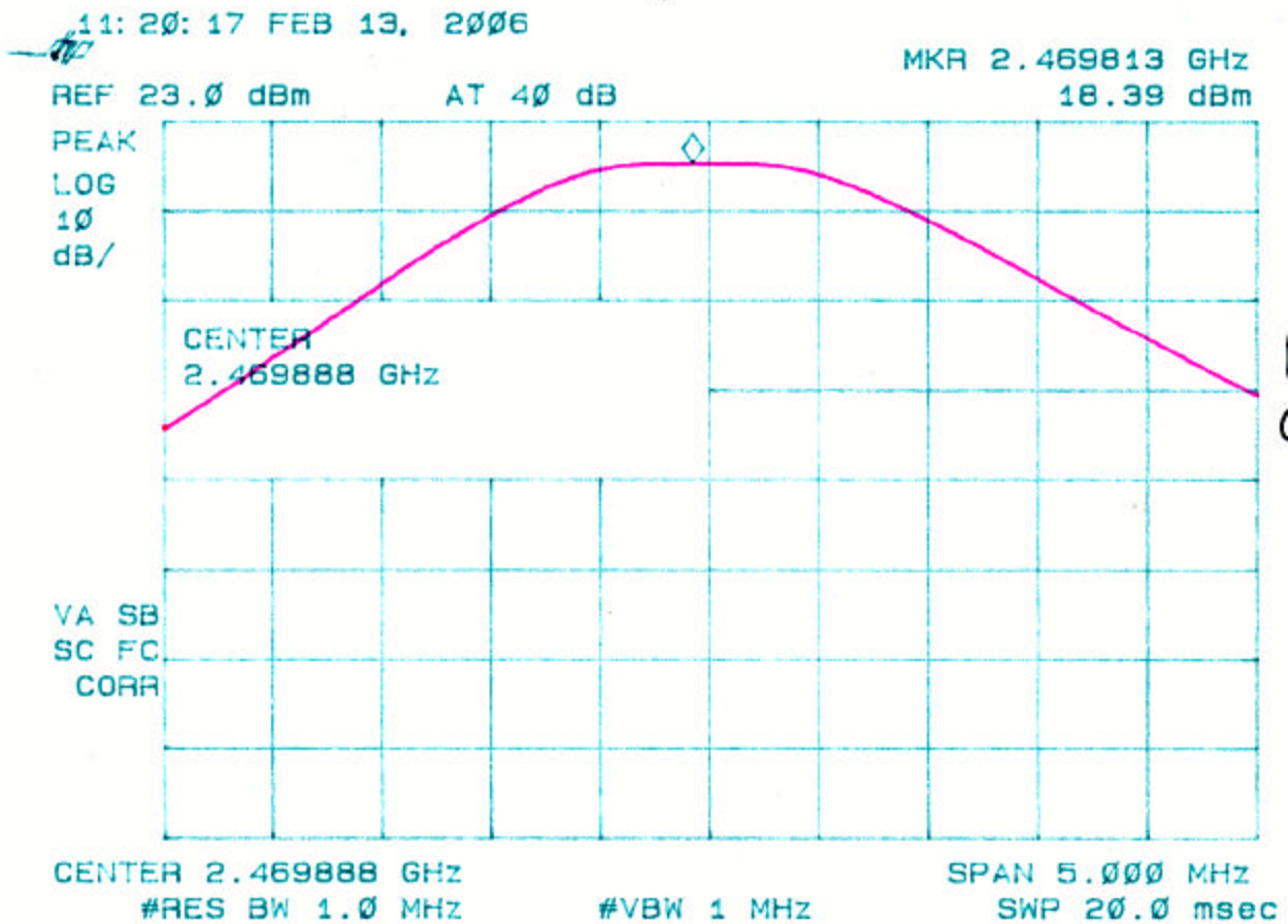
Figure 3c. Peak Power per FCC Section 15.247( b) High Channel
