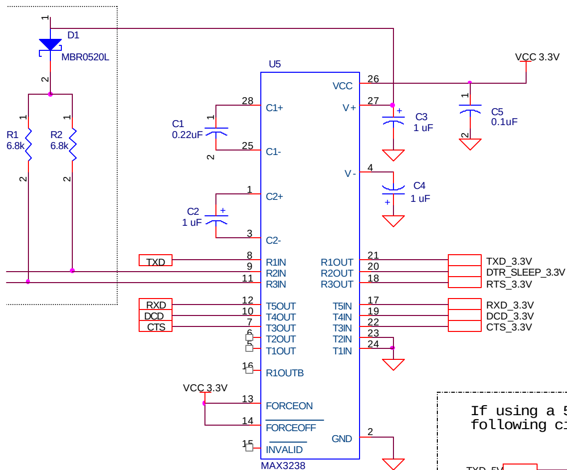
WIT2410 Interface
