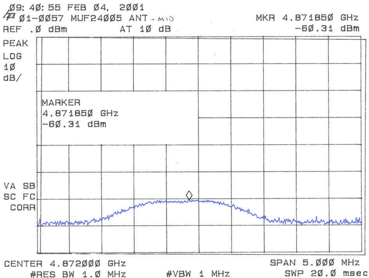
Figure 30 Peak Radiated Spurious Emission 15.247(c) Mid – MaxRad 5 dBi Whip
