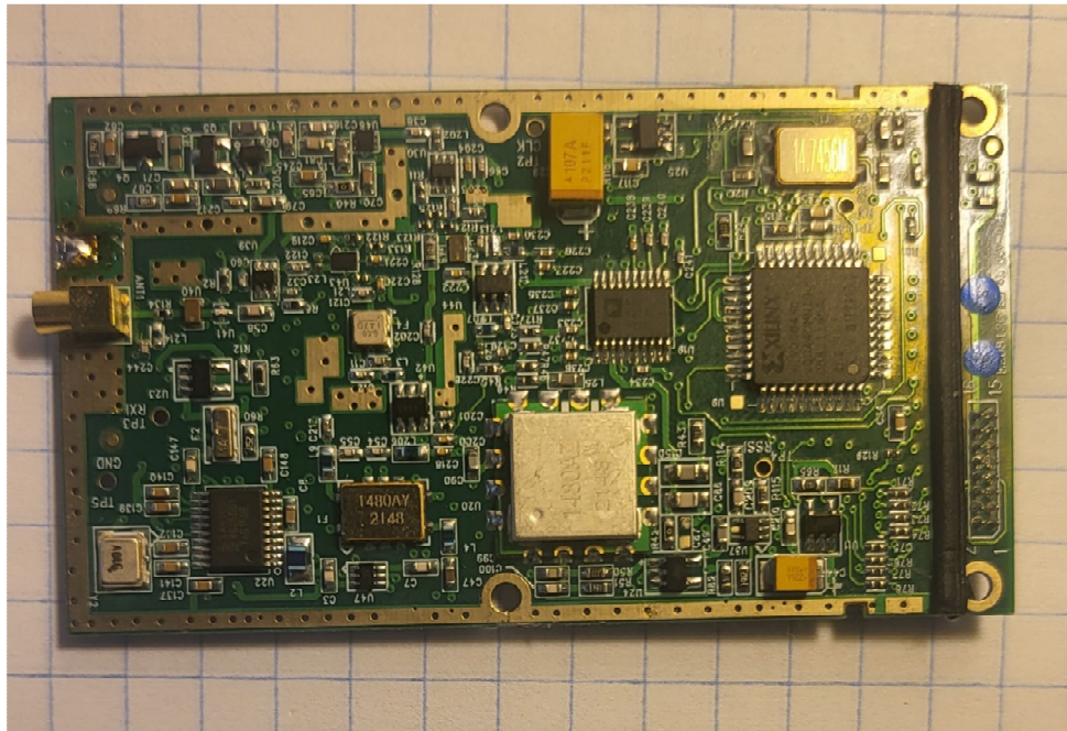
Figure 1. Top of PCB assembly
