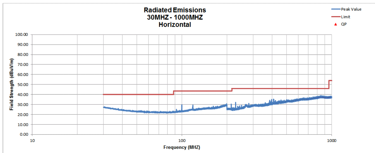
Figure 19. Horizontal Spurious Emissions, 30-1000 MHz
