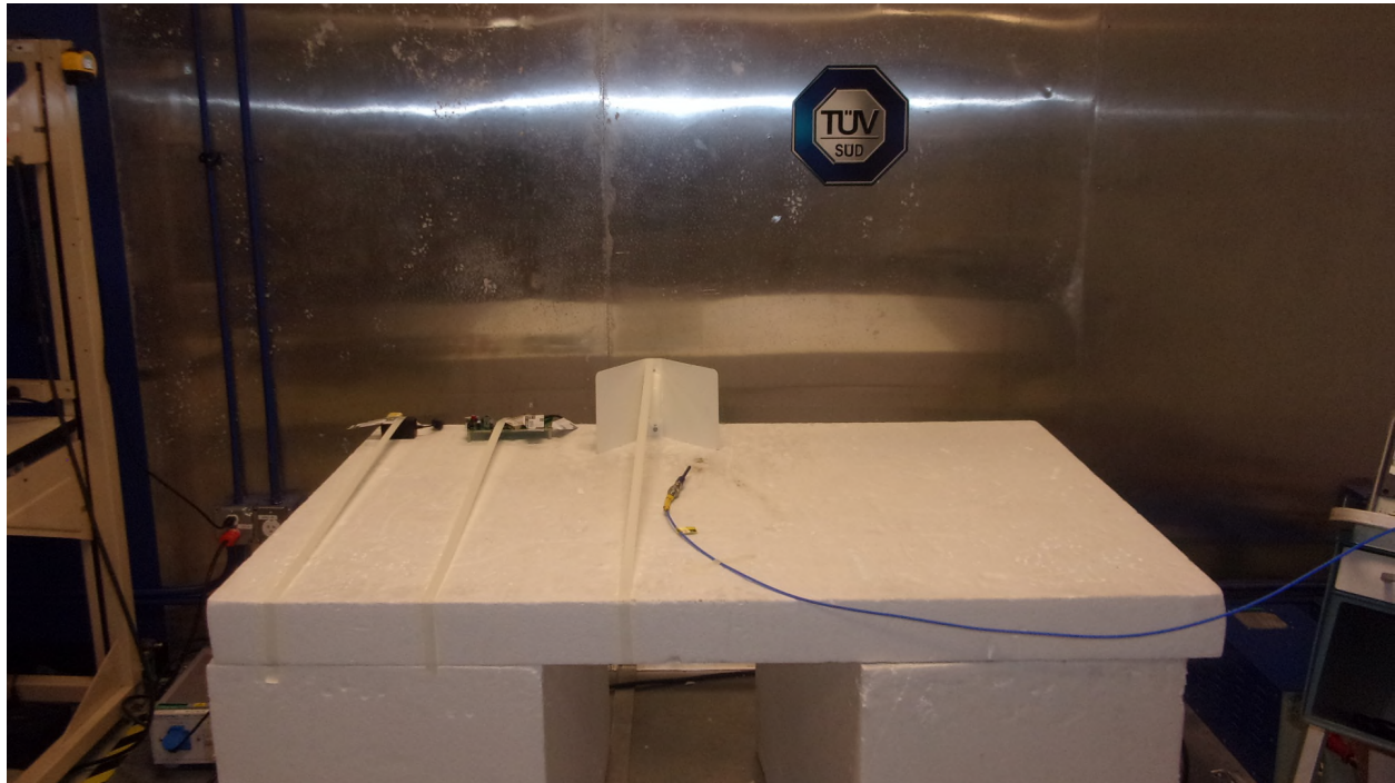
Figure 9: Equipment Under Test – AC Conducted Emissions
