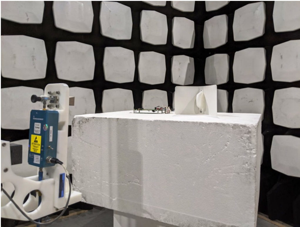
Figure 7: Equipment Under Test – Radiated Emissions – >18GHz
