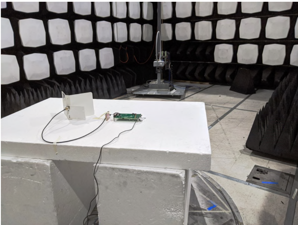
Figure 2: Equipment Under Test – Radiated Emissions – <30MHz
