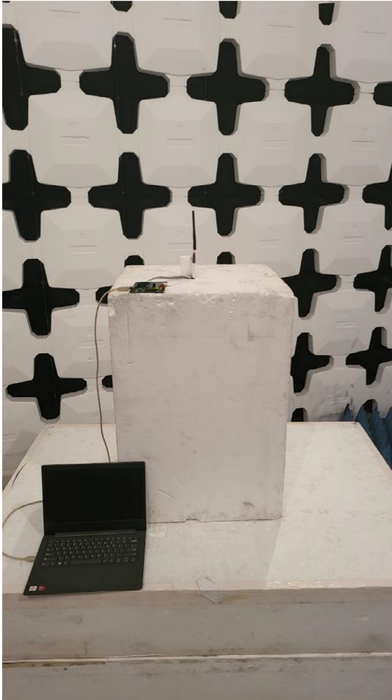
Figure 1. EUT Setup Fundamental Emissions, with Dipole
