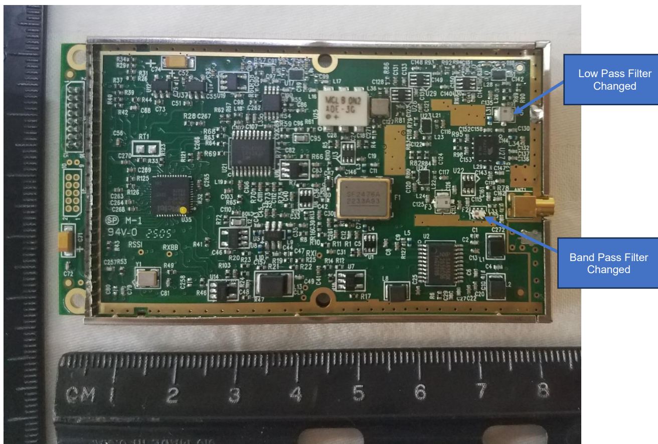
Figure 1. Main PCB with Shielding Removed.
