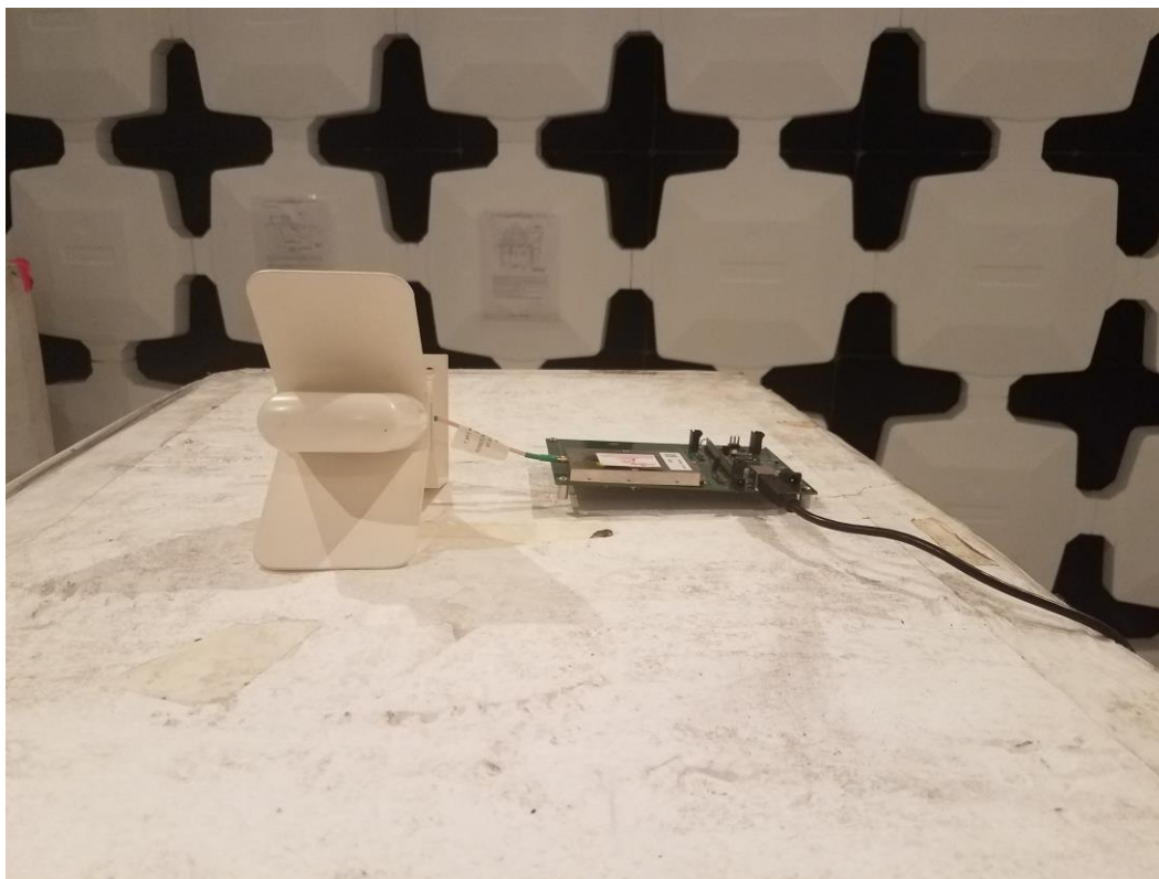
Figure 1. Radiated Emissions Test Setup, Corner Reflector Antenna
