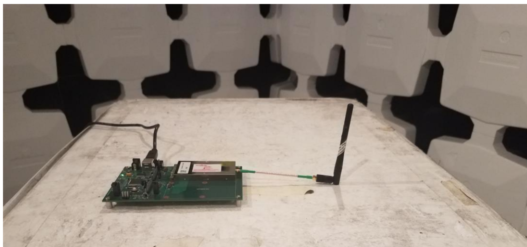
Figure 1. Radiated Emissions Test Setup, Dipole Antenna
