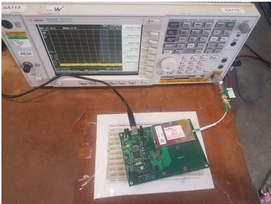
Figure 6. Conducted Emissions Test Setup
