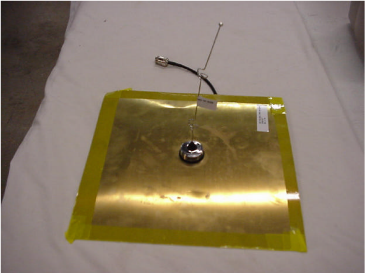
Photo 11. Whip Antenna
