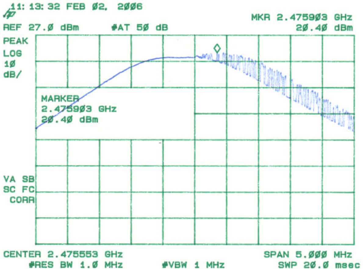
Figure 3d Conducted Power Peak High Channel Emission
