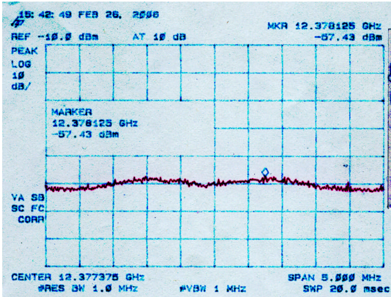
Figure 4u – 5 Peak Radiated Spurious Emission 15.247(c) High – Dipole Antenna
