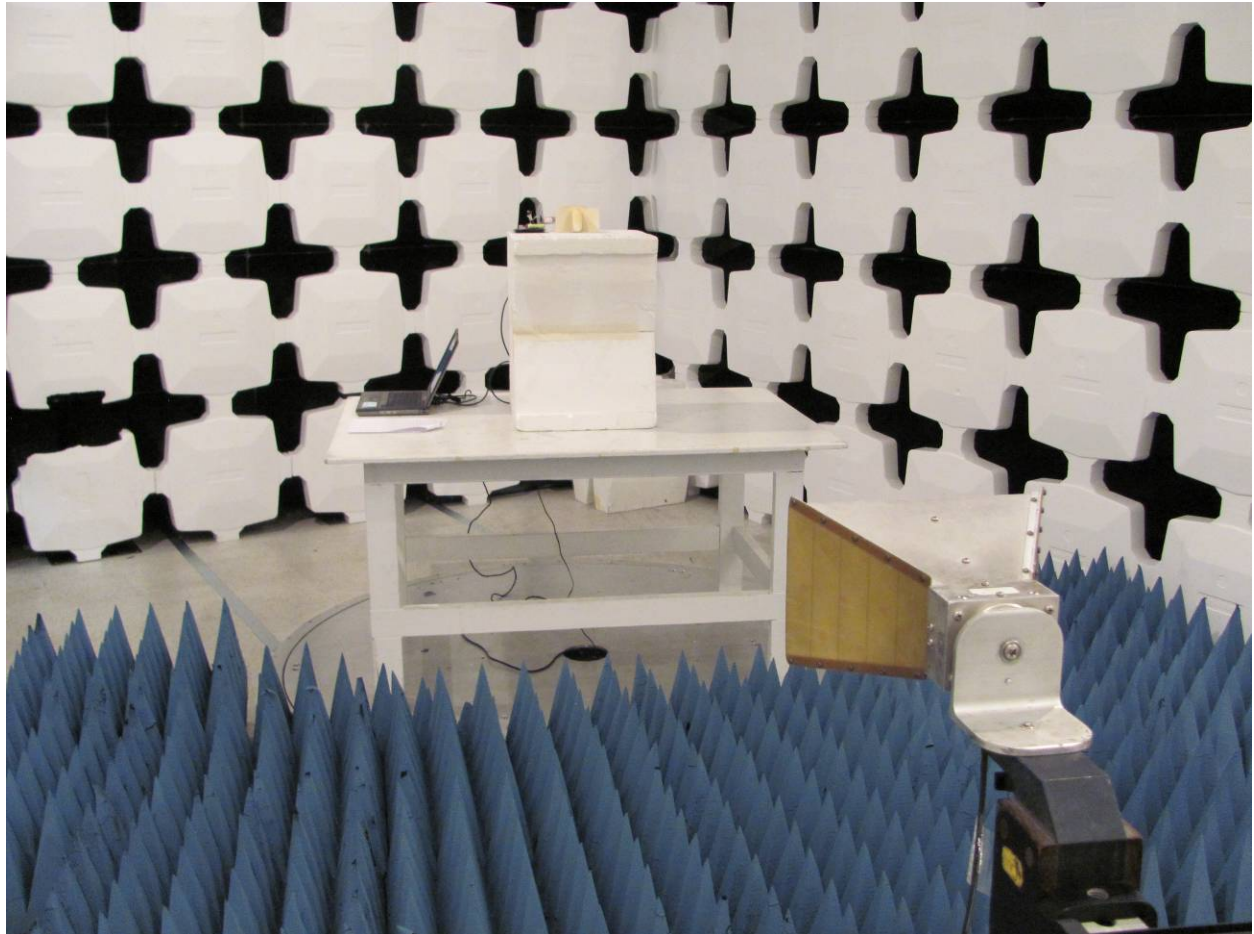
Figure 5. Radiated Emission Test Setup, Back, Corner Antenna
