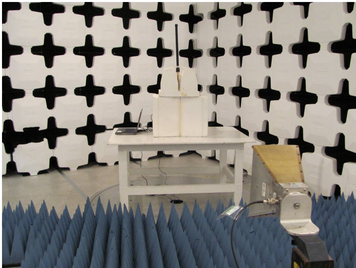
Figure 4. Radiated Emissions Test Setup, Back, Omni Antenna
