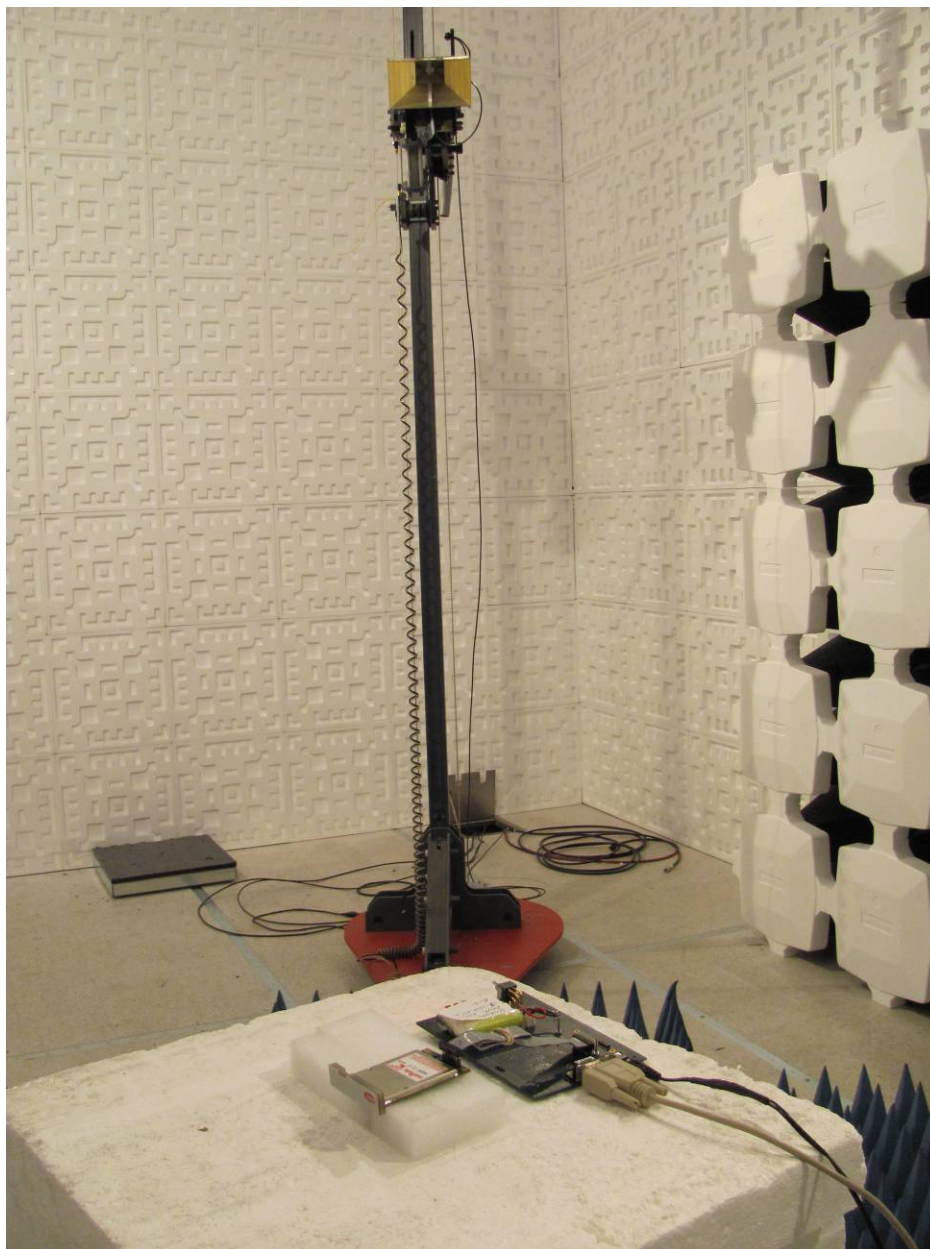
Figure 7. Radiated Emission Test Setup, Back. Patch Antenna
