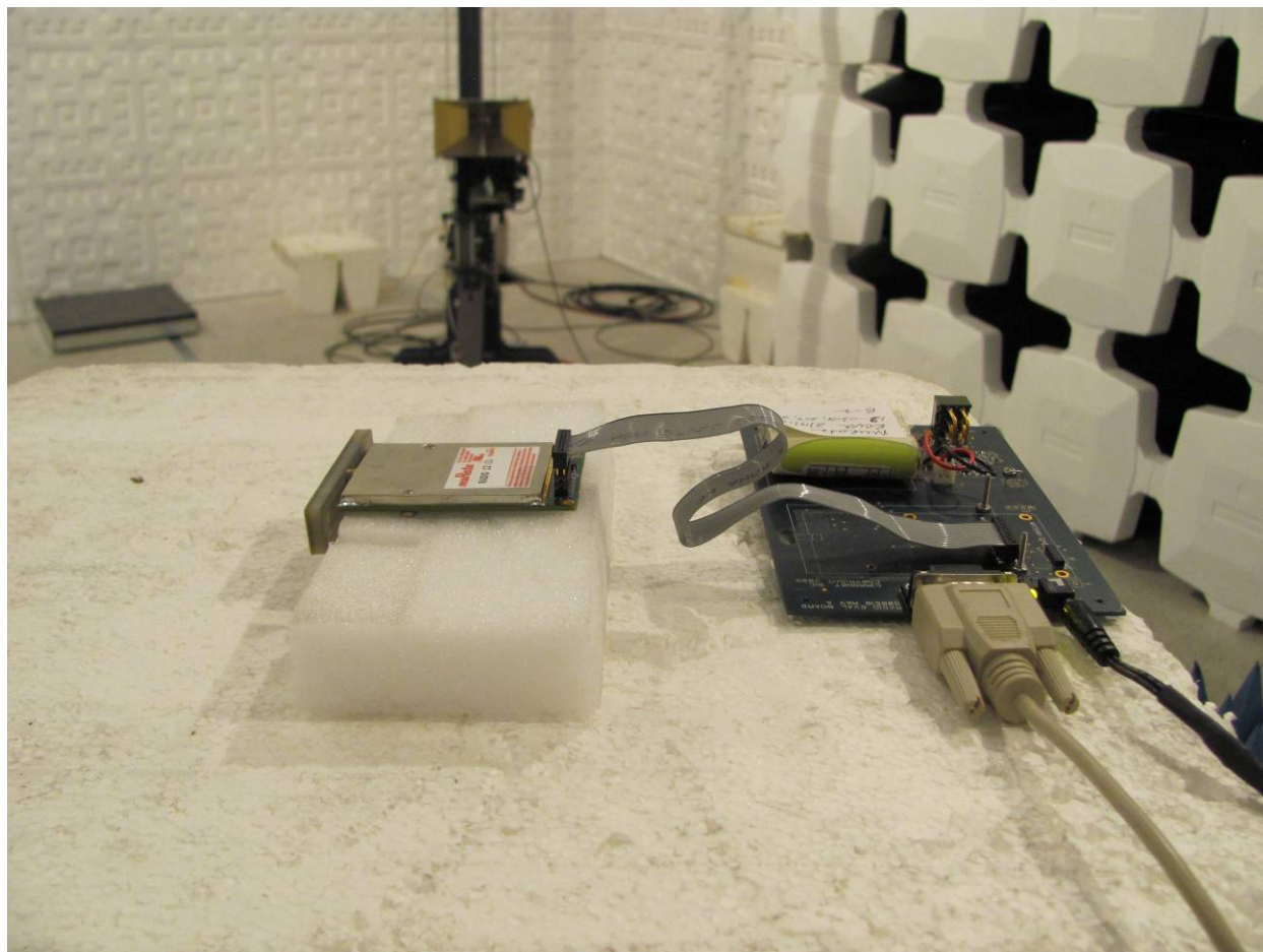
Figure 3. Radiated Emissions Test Setup, Front, Patch Antenna
