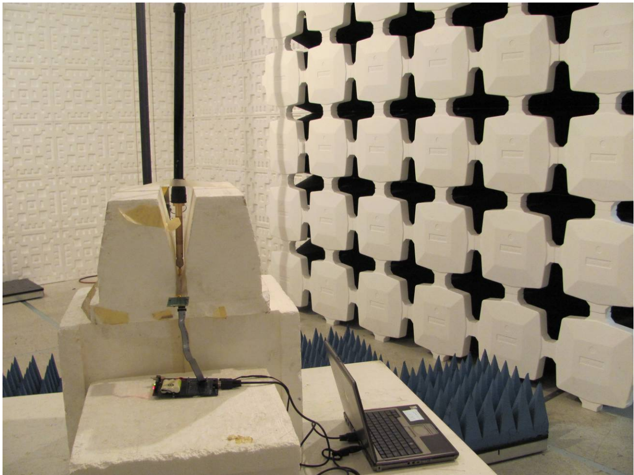
Figure 1. Radiated Emissions Test Setup, Front, Omni Antenna
