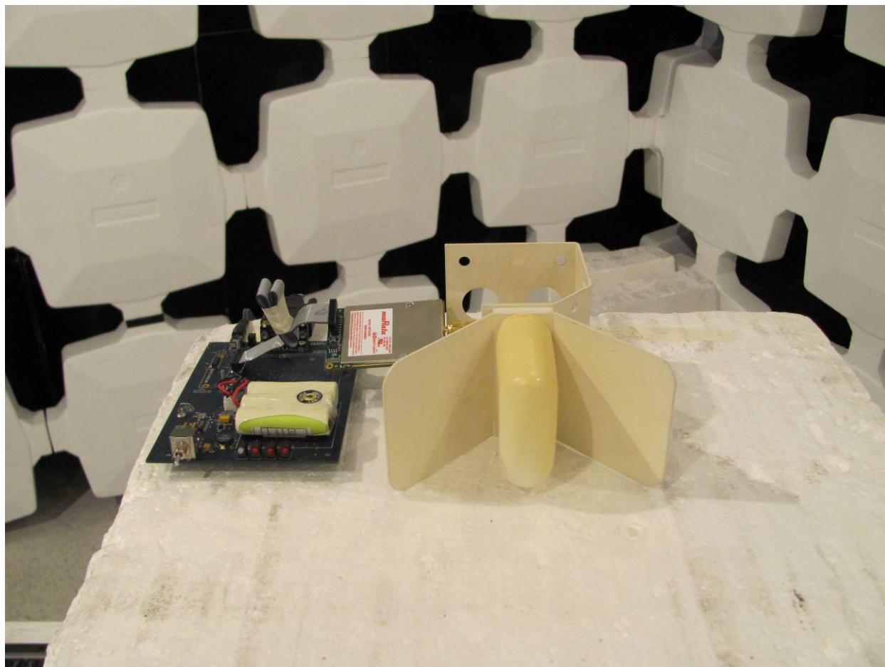
Figure 2. Radiated Emissions Test Setup, Front, Corner Antenna
