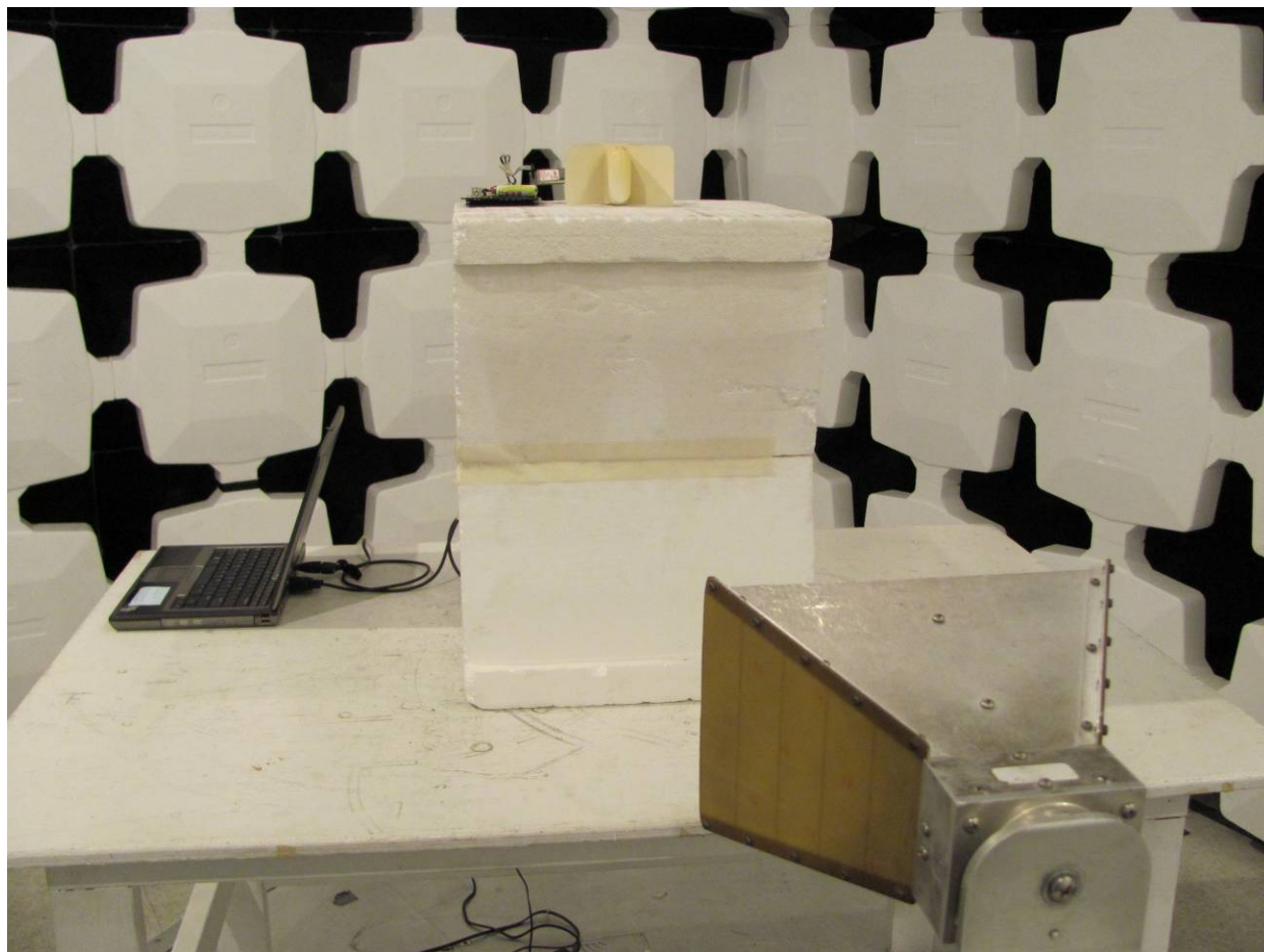
Figure 6. Radiated Emission Test Setup, 1 meter, Corner Antenna
