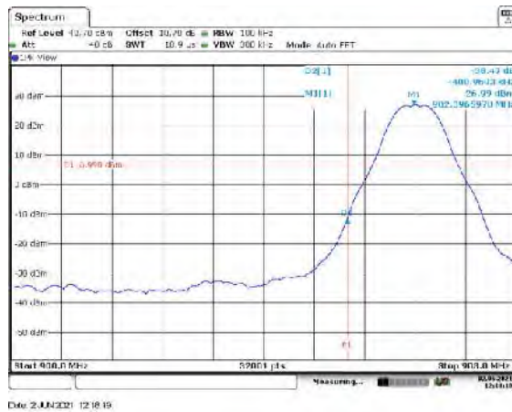
Figure 7.5.1.2-7: Lower Band edge – Mode 7
