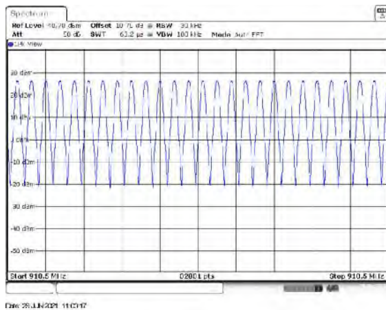
Figure 7.4.2.2-27: Mode 5 (83 Channels)
