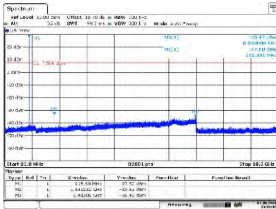
Figure 7.5.2.2-13: 30 MHz – 10 GHz – MCH-Mode 4
