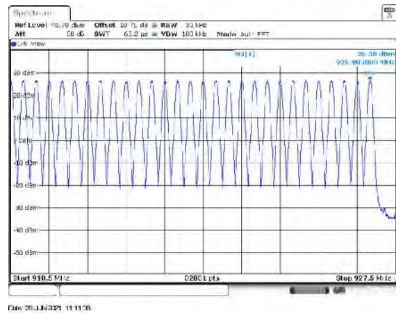
Figure 7.4.2.2-28: Mode 5 (83 Channels)
