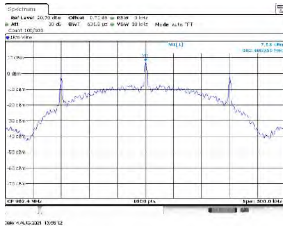
Figure 7.6.2.1-1: PSD – LCH-Mode 6
