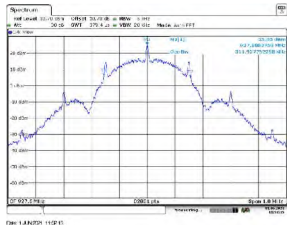
Figure 7.4.4.2-52: 99% BW High Channel – Mode 7
