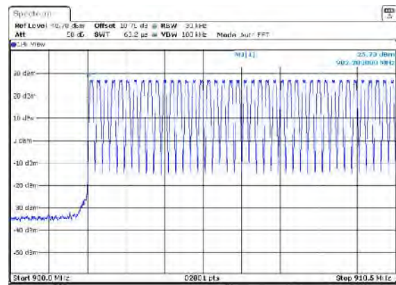
Figure 7.4.2.2-38: Mode 8 (512 Channels)
