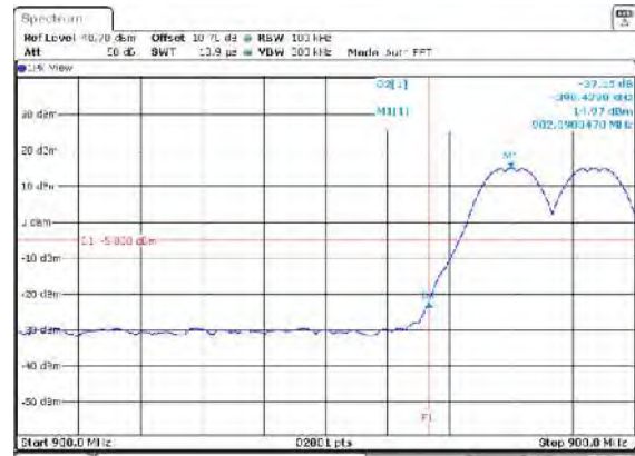
Figure 7.5.1.2-6: Lower Band edge – Mode 6
