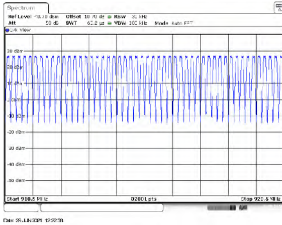
Figure 7.4.2.2-41: Mode 8 (129 Channels)
