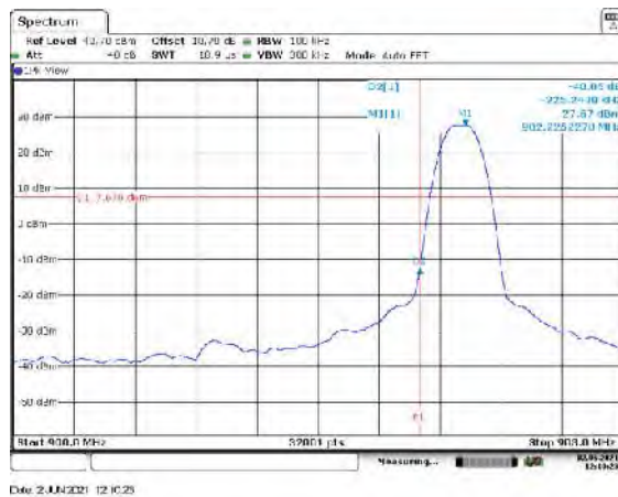
Figure 7.5.1.2-9: Lower Band edge – Mode 9
