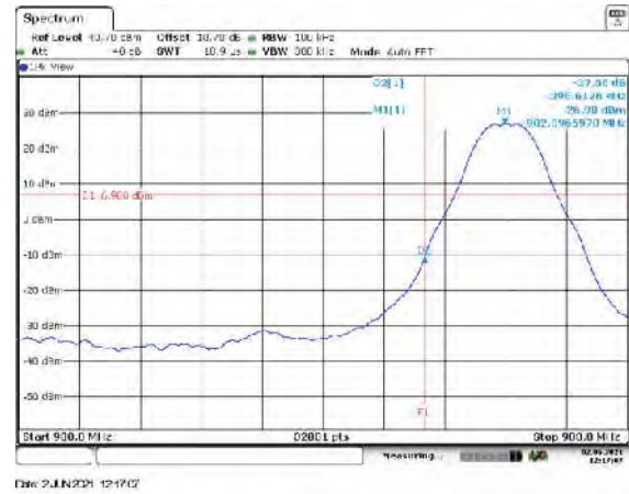
Figure 7.5.1.2-6: Lower Band edge – Mode 6
