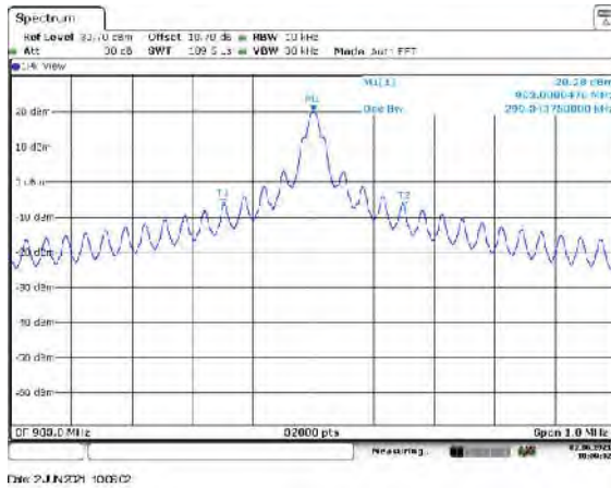
Figure 7.4.4.2-29: 99% BW Low Channel – Mode 2
