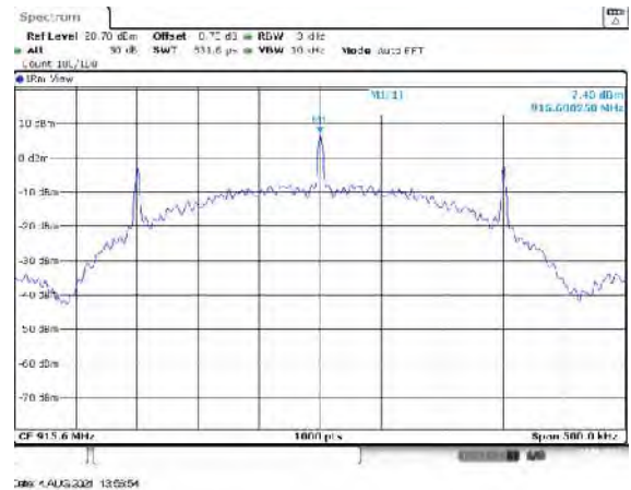
Figure 7.6.2.1-2: PSD – MCH-Mode 6
