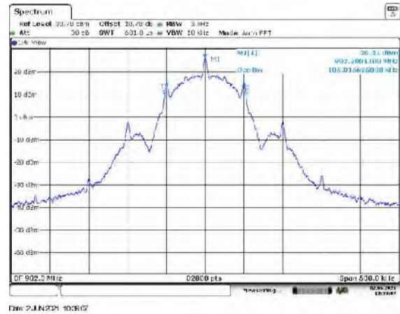
Figure 7.4.4.2-30: 99% BW Low Channel – Mode 3
