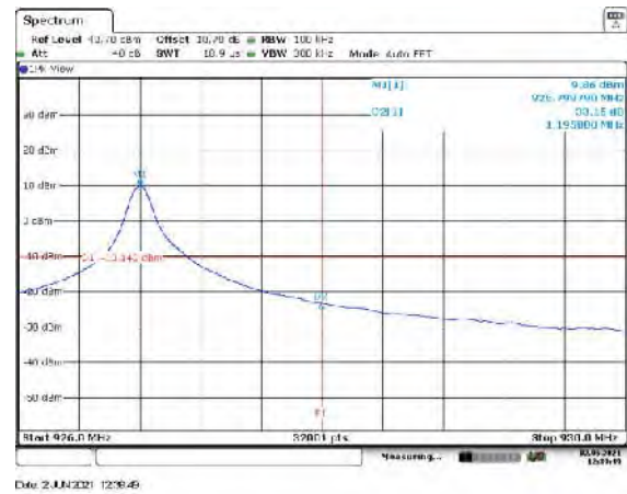
Figure 7.5.1.2-10: Upper Band edge – Mode 1
