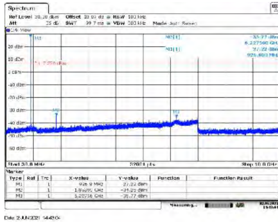
Figure 7.5.2.2-23: 30 MHz – 10 GHz – HCH-Mode 5
