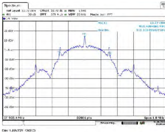
Figure 7.4.4.2-31: 99% BW Low Channel – mode 4
