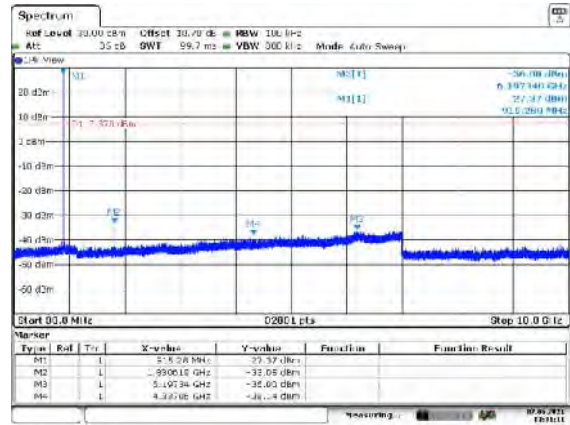
Figure 7.5.2.2-12: 30 MHz – 10 GHz – MCH-Mode 3
