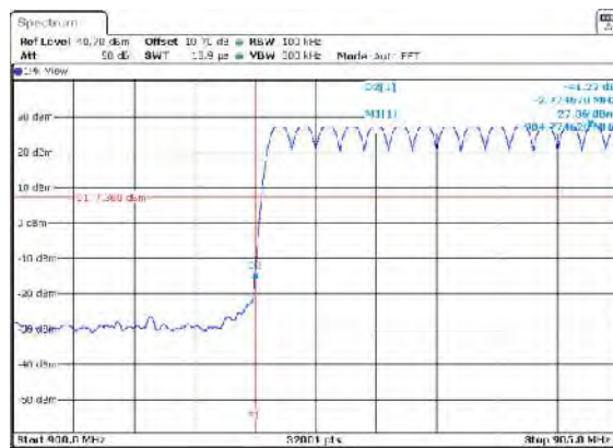
Figure 7.5.1.2-9: Lower Band edge – Mode 9
