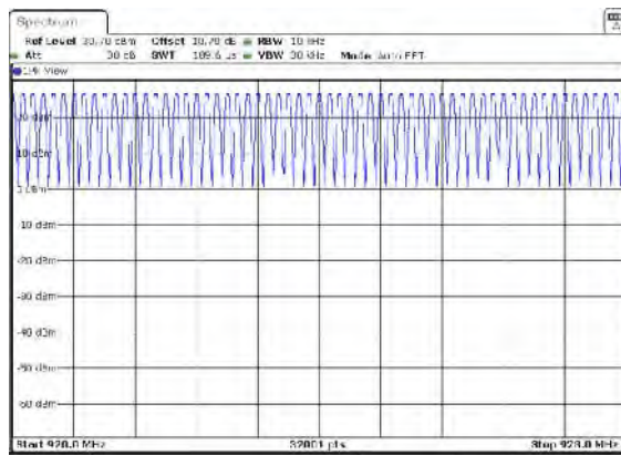
Figure 7.4.2.2-35: Mode 8 (512 Channels)
