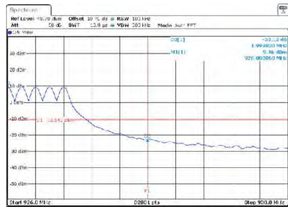
Figure 7.5.1.2-10: Upper Band edge – Mode 10
