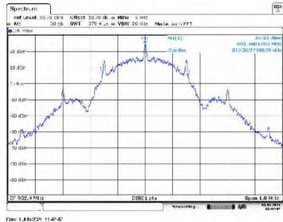
Figure 7.4.4.2-32: 99% BW Low Channel – Mode 5
