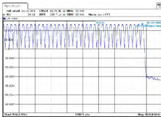
Figure 7.4.2.2-37: Mode 8 (512 Channels)
