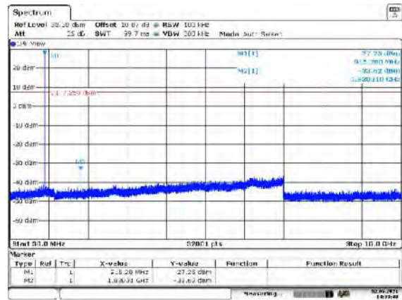
Figure 7.5.2.2-14: 30 MHz – 10 GHz – MCH-Mode 5
