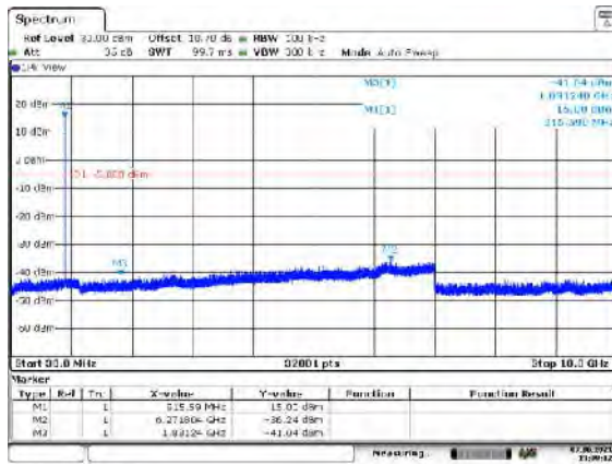
Figure 7.5.2.2-15: 30 MHz – 10 GHz – MCH-Mode 6
