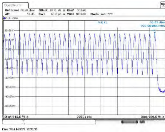
Figure 7.4.2.2-23: Mode 3 (512 Channels)
