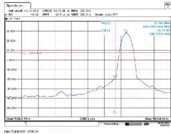
Figure 7.5.1.2-8: Lower Band edge – Mode 8
