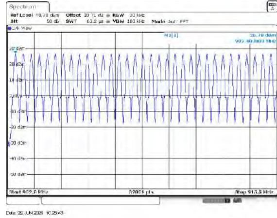
Figure 7.4.2.2-24: Mode 4 (64 Channels)
