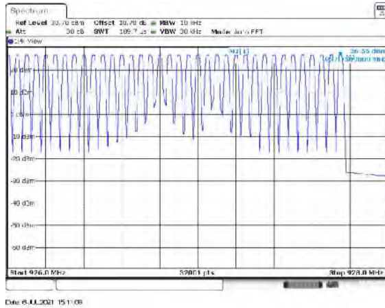
Figure 7.4.2.2-23: Mode 3 (512 Channels)
