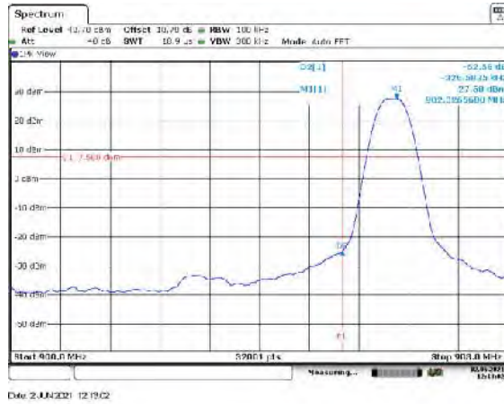
Figure 7.5.1.2-5: Lower Band edge – Mode 5
