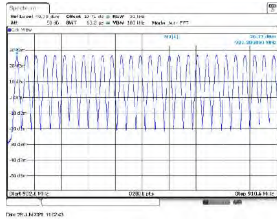
Figure 7.4.2.2-24: Mode 4 (64 Channels)
