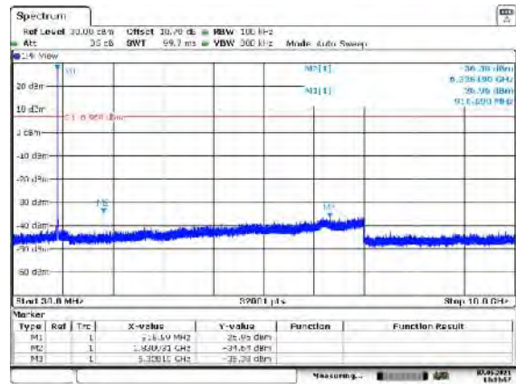
Figure 7.5.2.2-16: 30 MHz – 10 GHz – MCH-Mode 7
