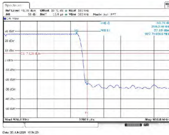
Figure 7.5.1.2-17: Upper Band edge – Mode 8
