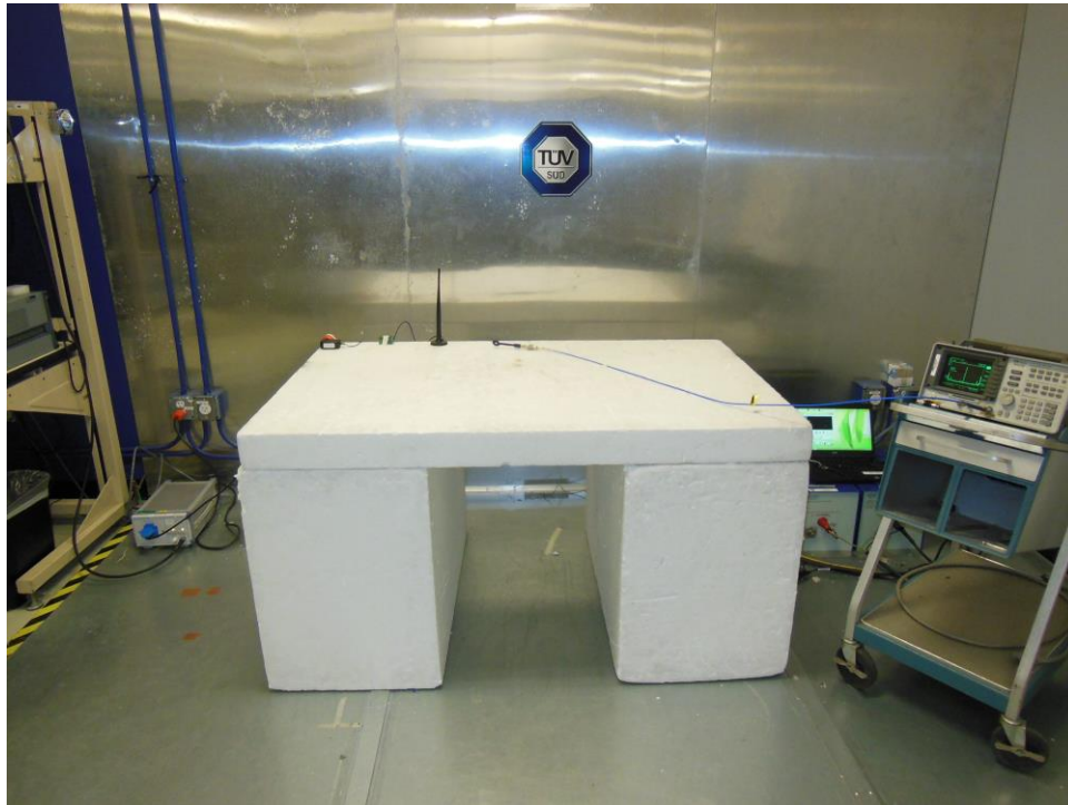
Figure 5: EUT - AC Power line Conducted Emissions
