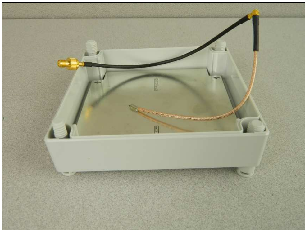
Figure 14: External Photo – Patch Antenna
