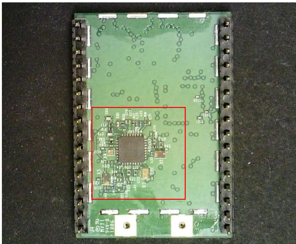
Figure 2. Bottom of Module with Shield removed
