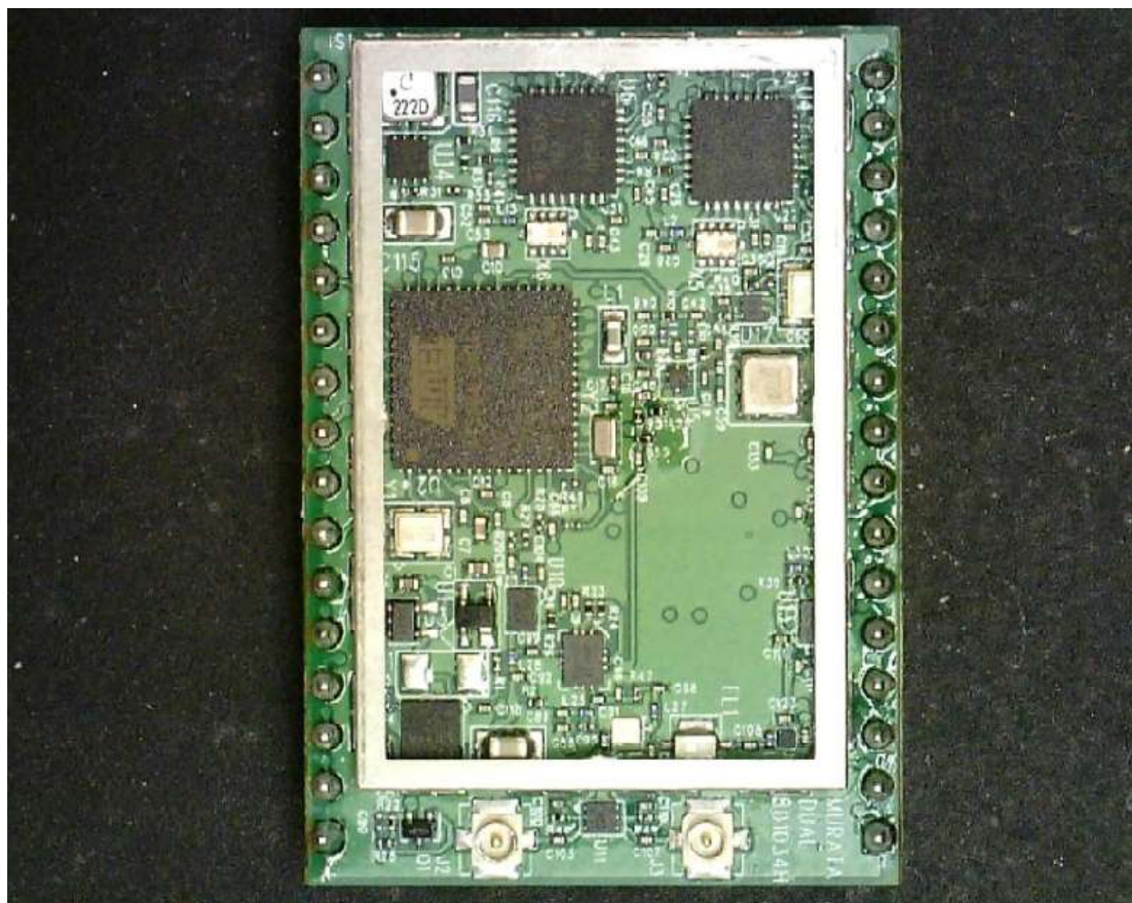
Figure 1. Top of Module with Shield Removed
