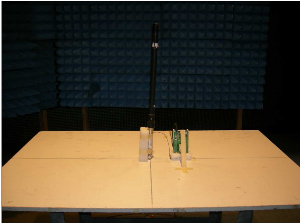
Figure 4: Radiated Emissions – Dipole Antenna
