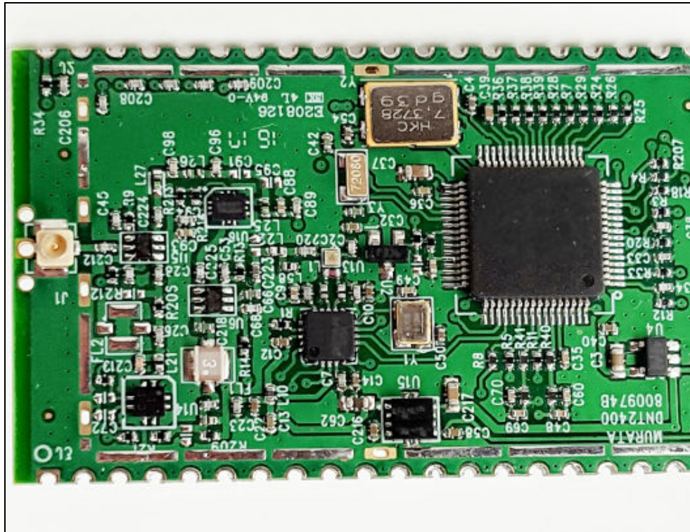
Figure 1: Internal Photo – DNT2400PC Shield Removed
