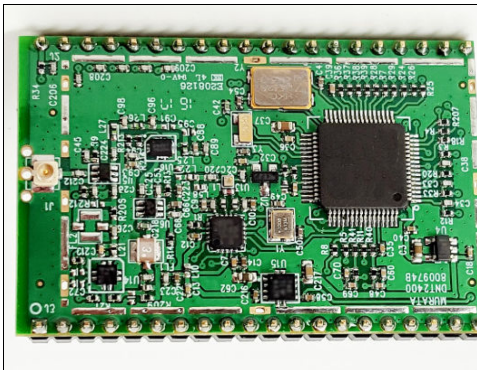
Figure 2: Internal Photo – DNT2400PP Shield Removed
