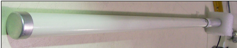
Figure 7: Dipole Antenna
