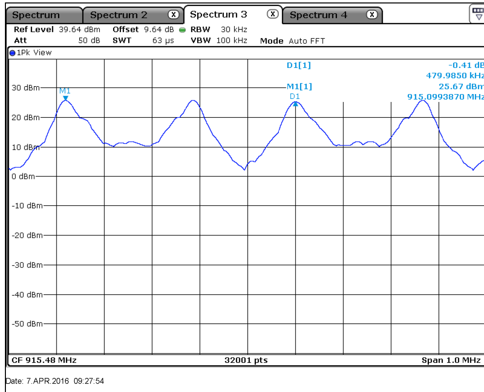
Figure 7.4.1.2-1: Frequency Separation
