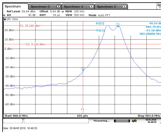
Figure 7.5.1.2-1: Lower BE
