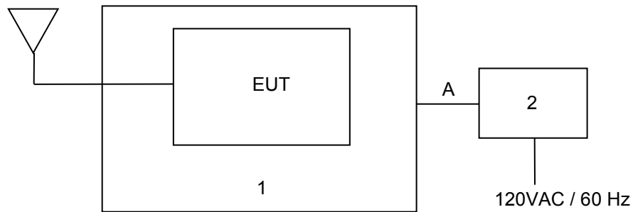
Figure 1: Radiated & AC Power Line Conducted Emissions Setup
