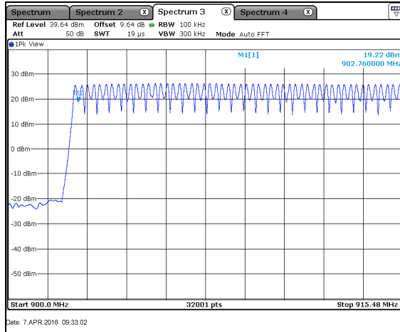
Figure 7.4.2.2-1: No. of Hopping Channels
