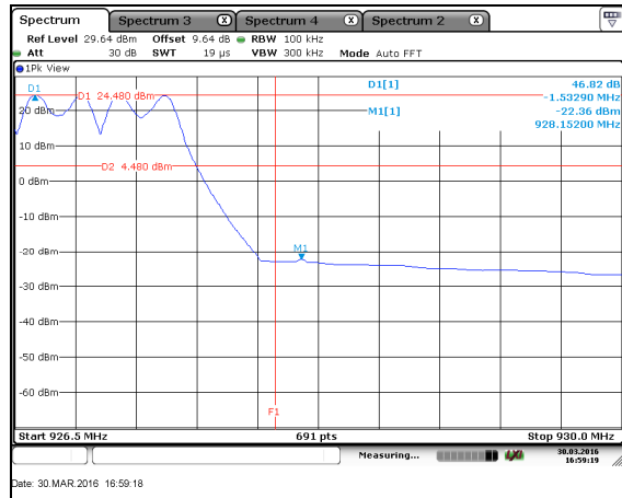
Figure 7.5.1.2-4: Upper BE Hopping
