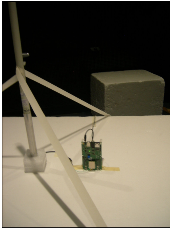
Figure 1: Radiated Emissions – Dipole Antenna
