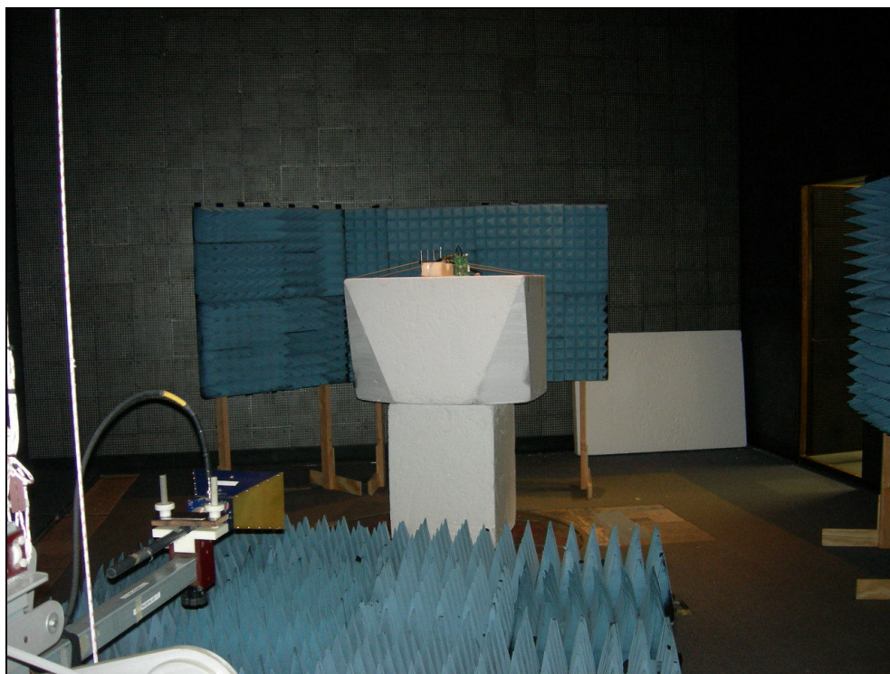
Figure 3: Radiated Emissions – Yagi Antenna
