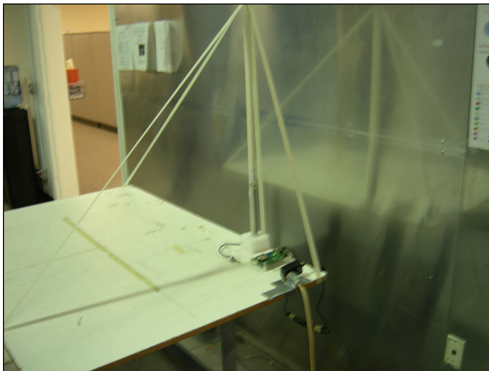
Figure 7: Conducted Emissions – Dipole Antenna
