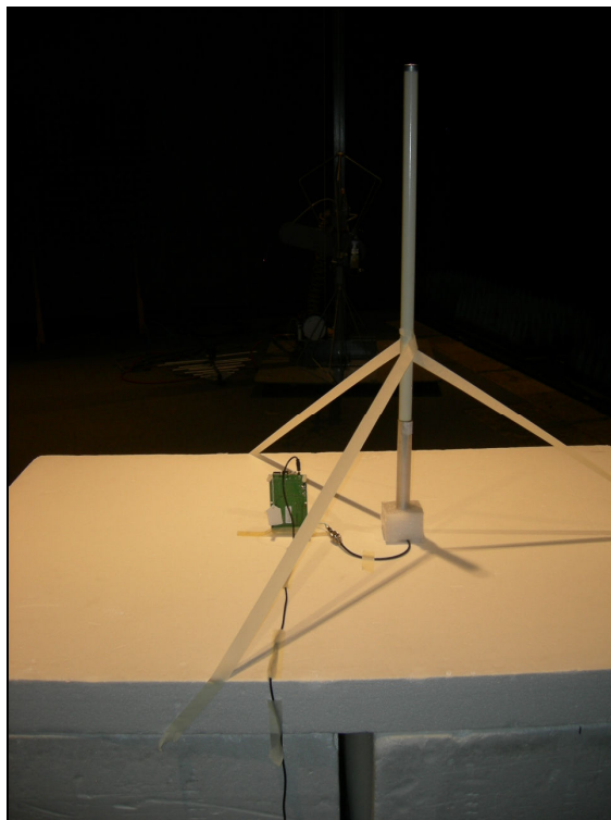
Figure 2: Radiated Emissions – Dipole Antenna
