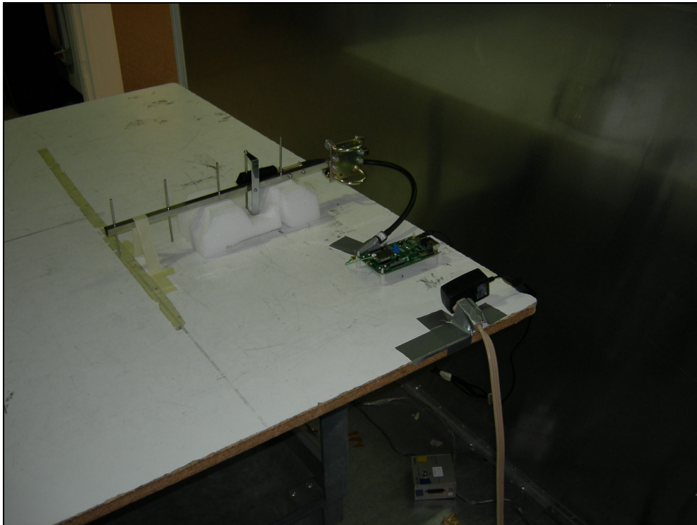
Figure 9: Conducted Emissions – Yagi Antenna
