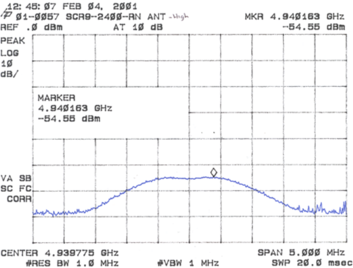
Figure 3k Peak Radiated Spurious Emission 15.247(c) High– Mobile Mark 9 dBi Corner Reflector
