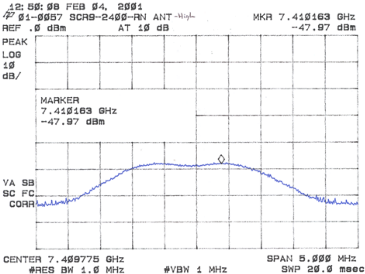
Figure 3l Peak Radiated Spurious Emission 15.247(c) High– Mobile Mark 9 dBi Corner Reflector
