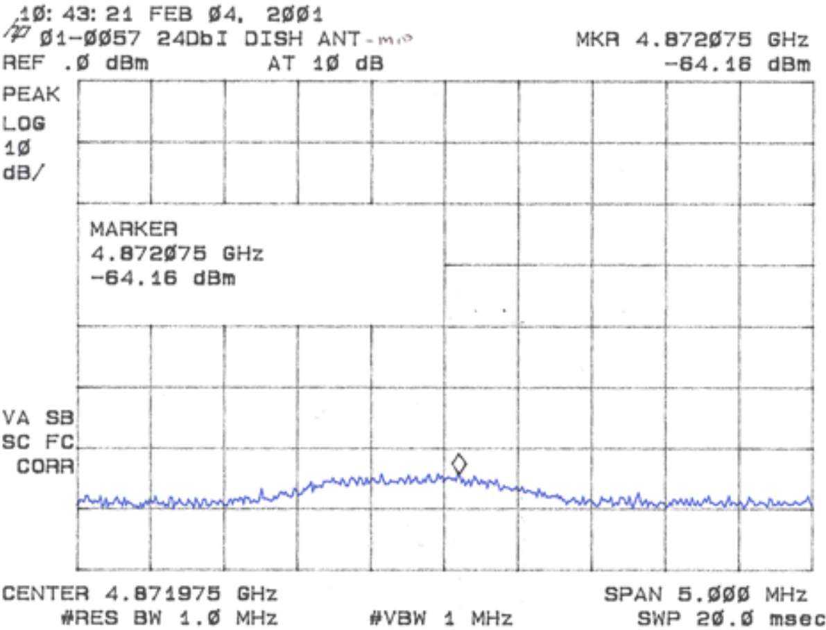
Figure 3u Peak Radiated Spurious Emission 15.247(c) Mid – Andrews 24 dBi Parabolic Dish
