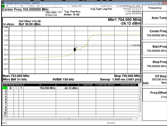
Cat M1 Band17 5MHz 16QAM 6 0 LowCH23755
