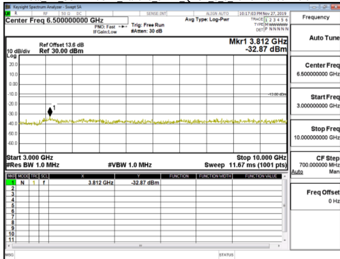
Cat M1 3GHz~10GHz Band13 5MHz 16QAM 6 0 LowCH23205-779.5
