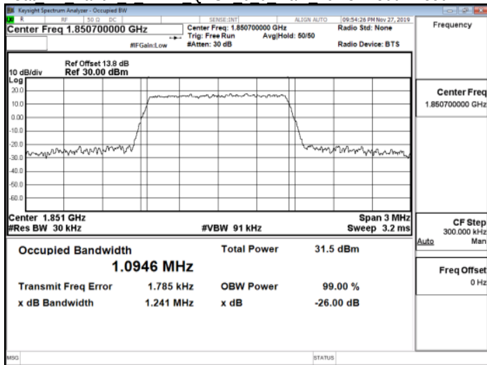
Cat M1 Band2 1 4MHz 16QAM 6 0 Main LowCH18607-1850.7
