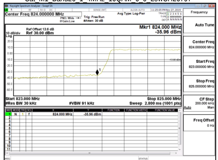
Cat M1 Band26 1 4MHz 16QAM 6 0 LowCH26797
