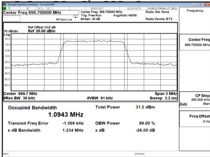
Cat M1 Band12 1 4MHz 16QAM 6 0 Main LowCH23017-699.7
