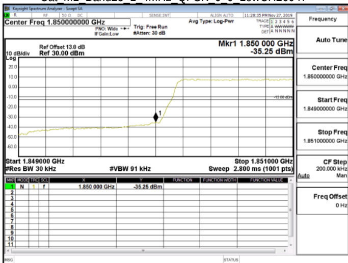
Cat M1 Band25 1 4MHz QPSK 6 0 LowCH26047
