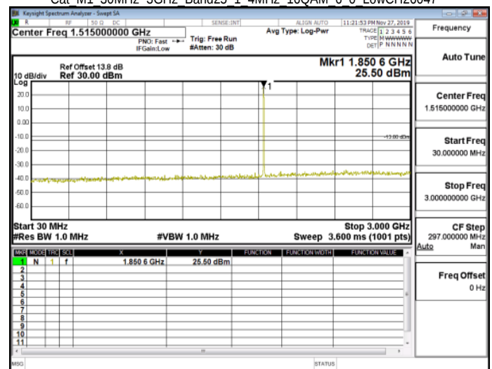
Cat M1 30MHz~3GHz Band25 1.4MHz 16QAM 6 0 LowCH26047
