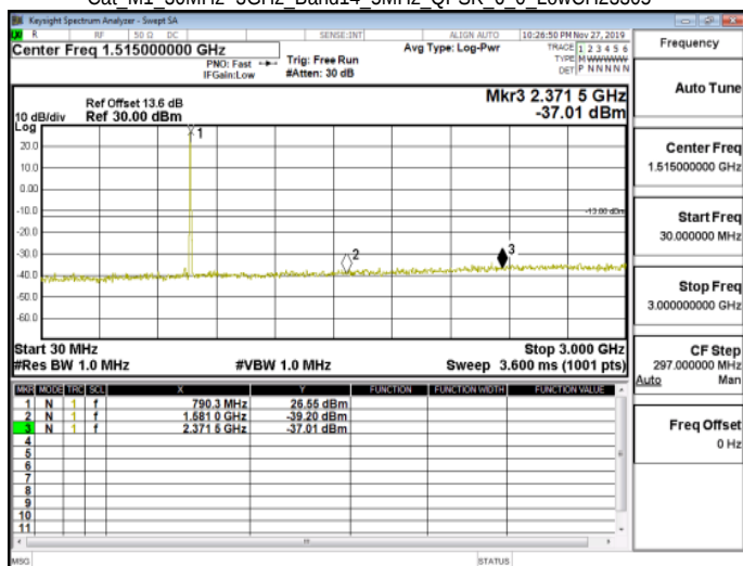
Cat M1 30MHz~3GHz Band14 5MHz QPSK 6 0 LowCH23305
