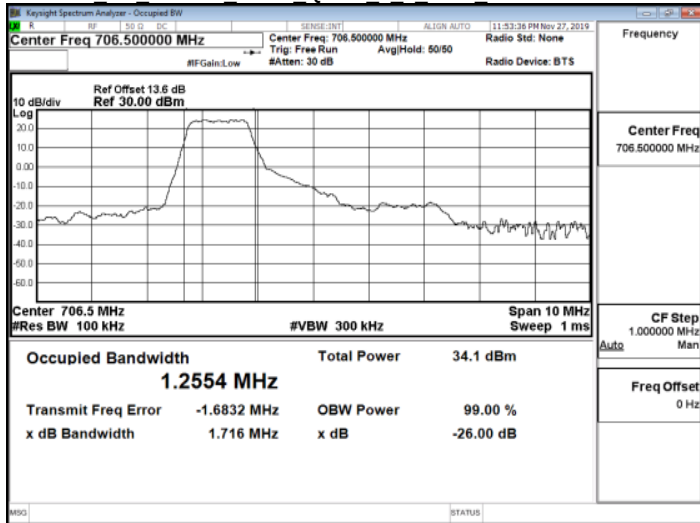
Cat M1 Band17 5MHz 16QAM 6 0 Main LowCH23755
