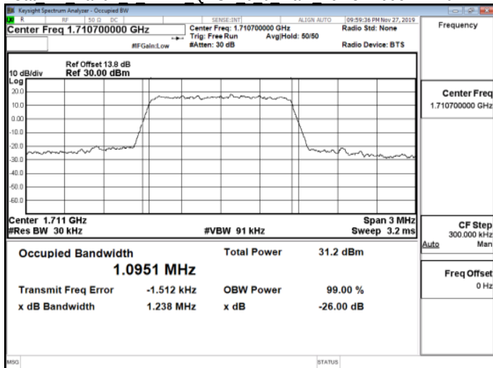
Cat M1 Band4 1 4MHz QPSK 6 0 Main LowCH19957-1710.7
