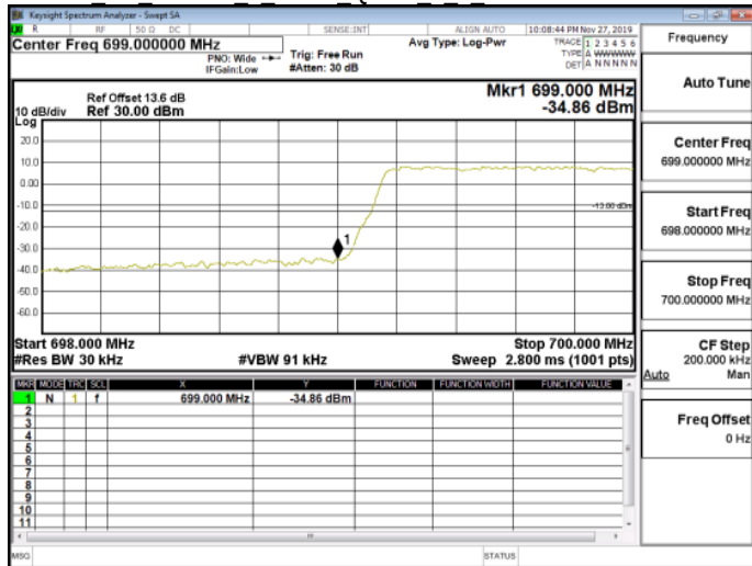
Cat M1_Band12 1 4MHz 16QAM 6 0 LowCH23017-699.7
