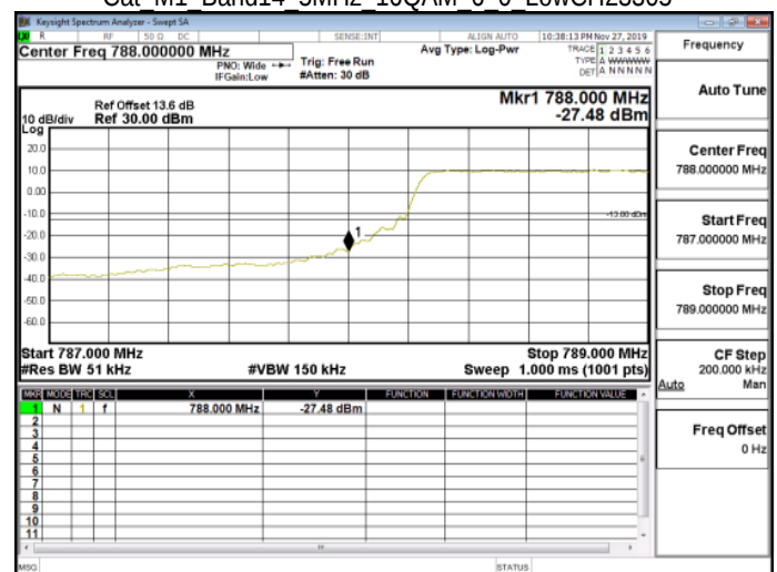
Cat M1_Band14 5MHz 16QAM 6 0 LowCH23305
