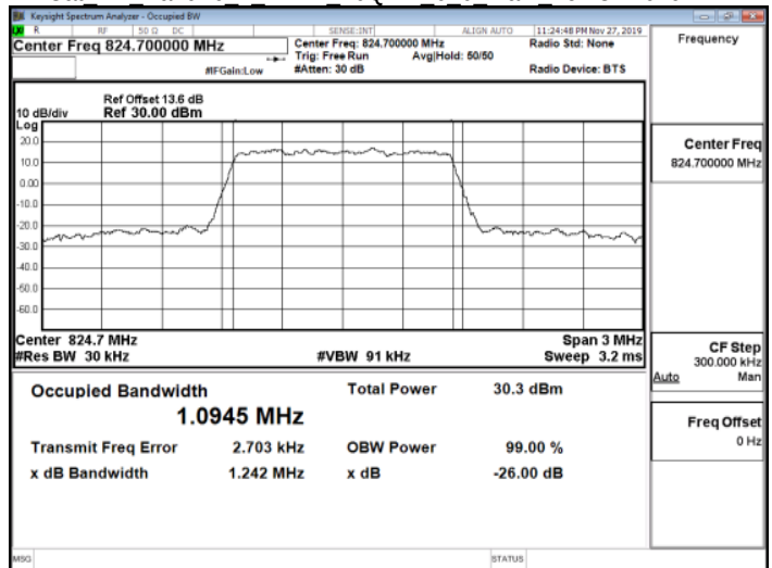
Cat M1 Band26 1 4MHz 16QAM 6 0 Main LowCH26797
