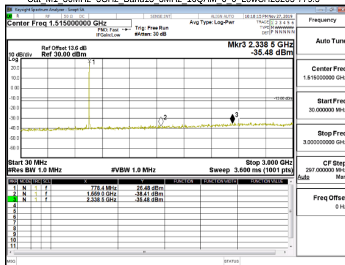
Cat M1 30MHz-3GHz Band13 5MHz 16QAM 6 0 LowCH23205-779.5
