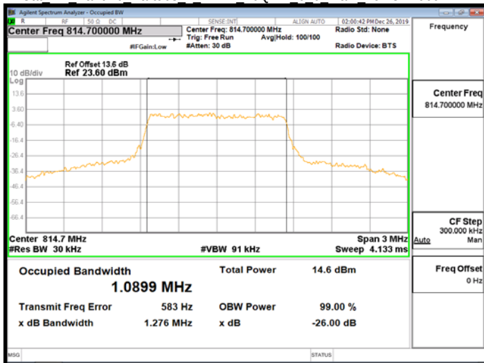
Cat M1 Band26 Part90s 1 4MHz 16QAM 6 0 Main LowCH26697
