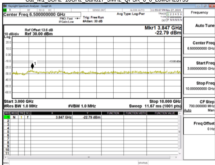
Cat M1 3GHz~10GHz Band17 5MHz QPSK 6 0 LowCH23755
