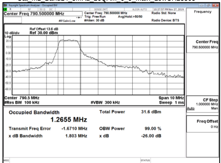
Cat M1 Band14 5MHz 16QAM 6 0 Main LowCH23305
