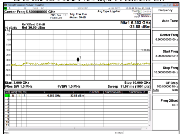
Cat M1 3GHz-10GHz Band5 1 4MHz 16QAM 6 0 LowCH20407-824.7
