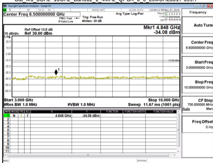
Cat M1 3GHz-10GHz Band12 1 4MHz QPSK 6 0 LowCH23017-699.7
