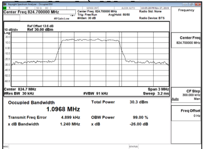
Cat M1 Band5 1 4MHz 16QAM 6 0 Main LowCH20407-824.7
