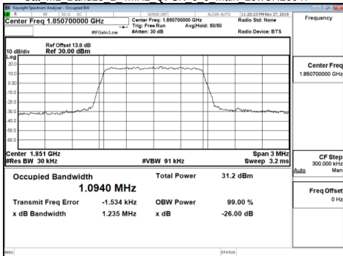
Cat M1 Band25 1 4MHz QPSK 6 0 Main LowCH26047
