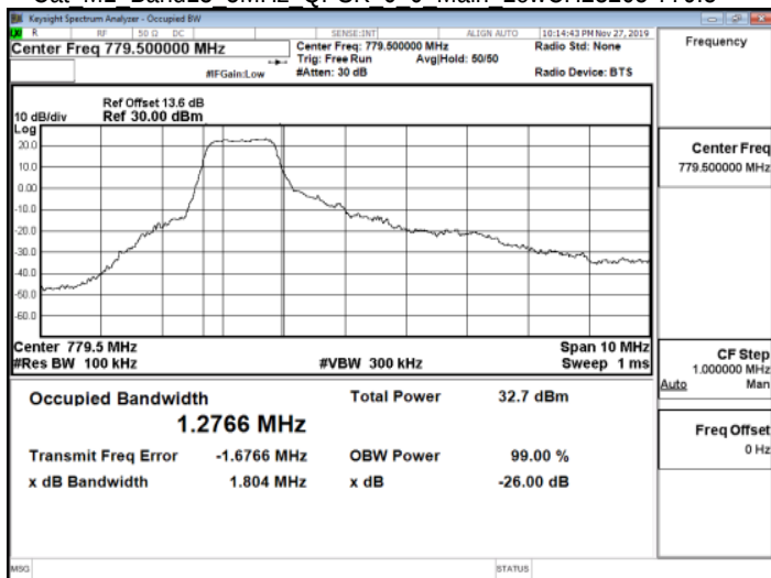
Cat M1 Band13 5MHz QPSK 6 0 Main LowCH23205-779.5
