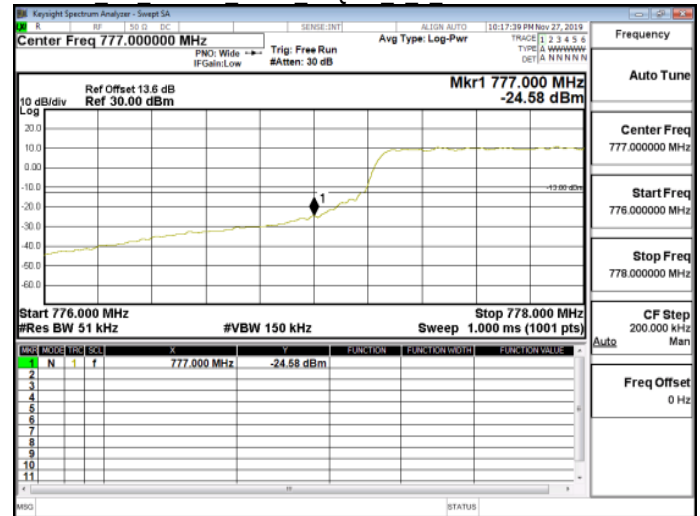
Cat M1_Band14 5MHz QPSK 6 0 LowCH23305
