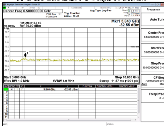
Cat M1 3GHz~10GHz Band26 1 4MHz 16QAM 6 0 LowCH26797
