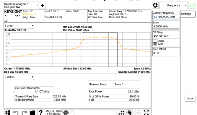
Cat-M1 Band66_3MHz_16QAM_RB6_0_CH132657
