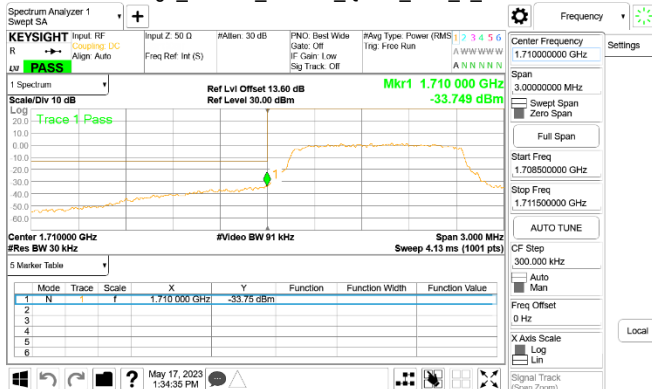
Band Edge_Band66_1.4MHz_QPSK_RB6_0_CH131979
