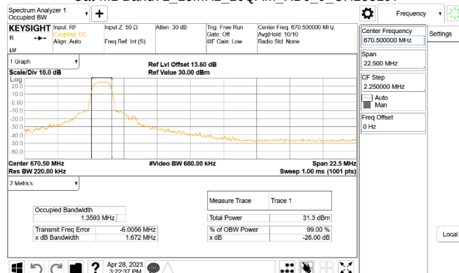
Cat-M1 Band71_15MHz_16QAM_RB6_0_CH133297
