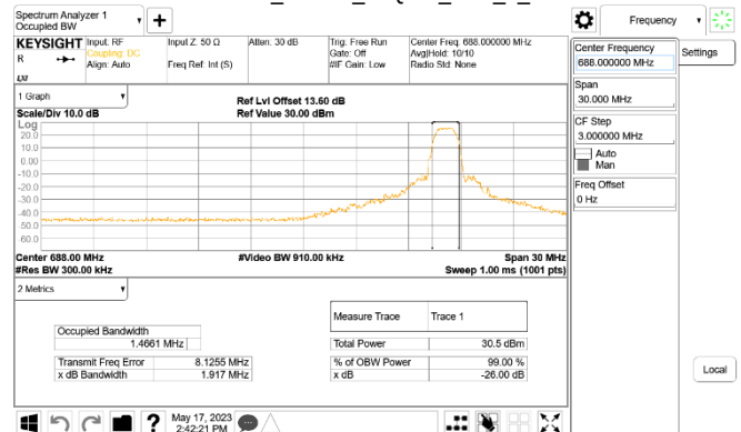
Cat-M1 Band71_20MHz_16QAM_RB6_0_CH133372
