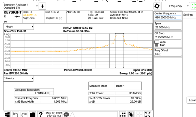
Cat-M1 Band71_15MHz_16QAM_RB6_0_CH133397
