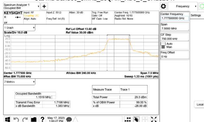
Cat-M1 Band66_5MHz_16QAM_RB6_0_CH132647
