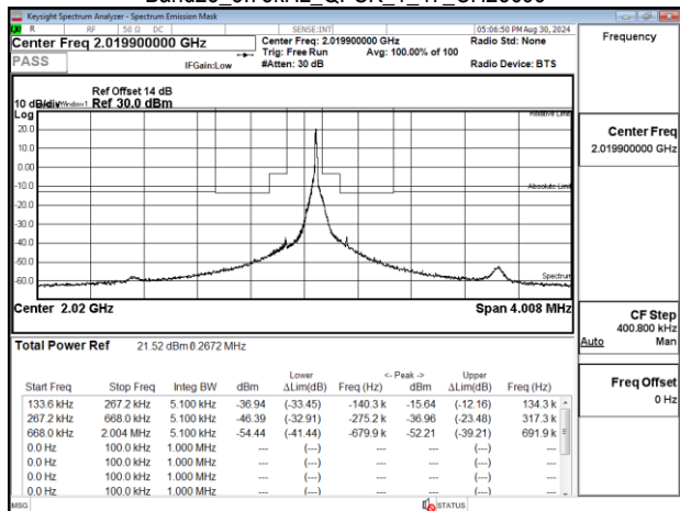
Band23 3.75kHz QPSK 1 47 CH25699
