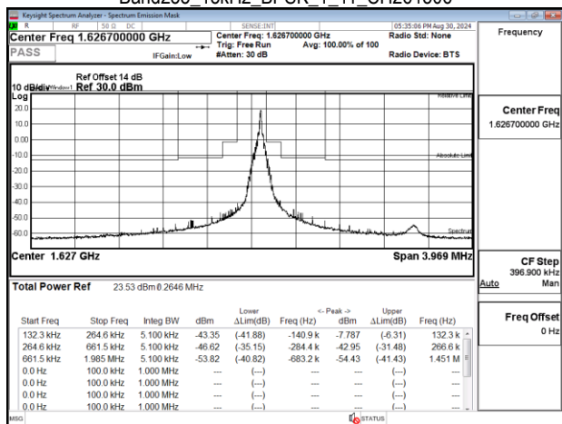
Band255 15kHz BPSK 1 11 CH261672
