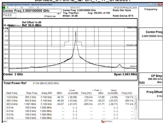
Band23 3.75kHz QPSK 1 47 CH25600
