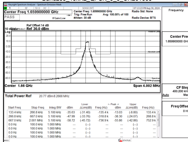
Band255_15kHz_QPSK_6_6_CH261838
