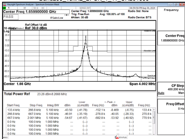
Band255 15kHz BPSK 1 11 CH261838
