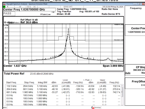
Band255 15kHz QPSK 1_11_CH261672
