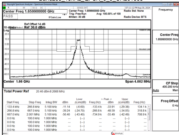
Band255_15kHz_QPSK_6_0_CH261838
