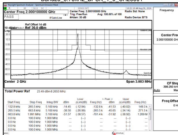
Band23 3.75kHz BPSK 1 0 CH25600
