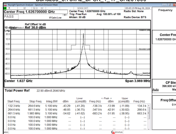
Band255 3.75kHz BPSK 1 47 CH261672
