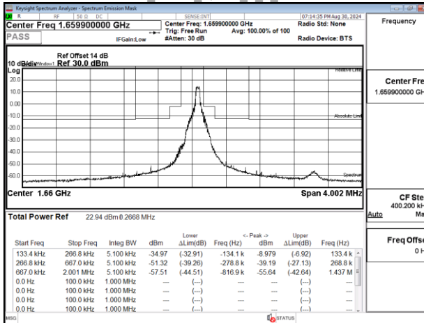
Band255_15kHz_QPSK_3_9_CH261838
