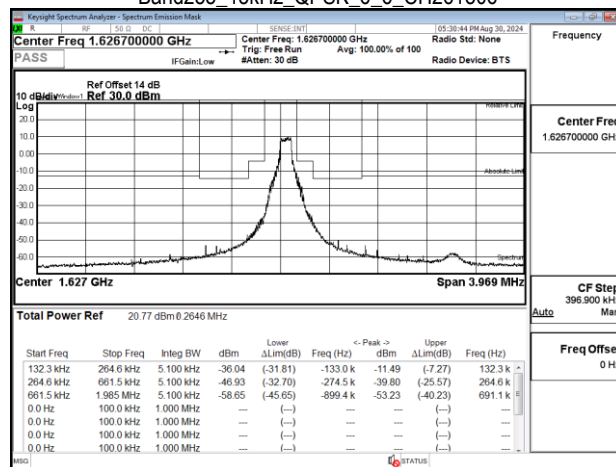
Band255_15kHz_QPSK_6_6_CH261672
