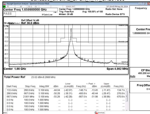
Band255 3.75kHz BPSK 1 47 CH261838
