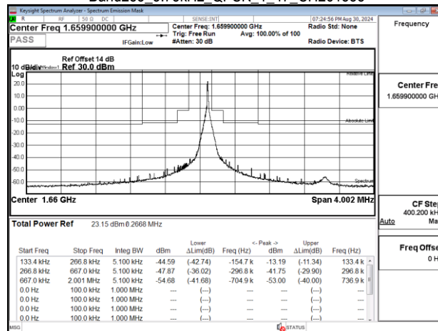
Band255 3.75kHz QPSK 1_47 CH261838
