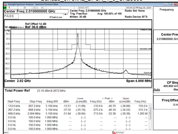
Band23 3.75kHz BPSK 1 0 CH25699
