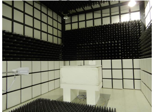
Part_25_Radiated_Setup
