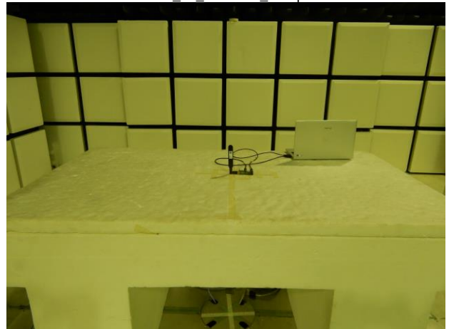
Part_25_Radiated_Setup
