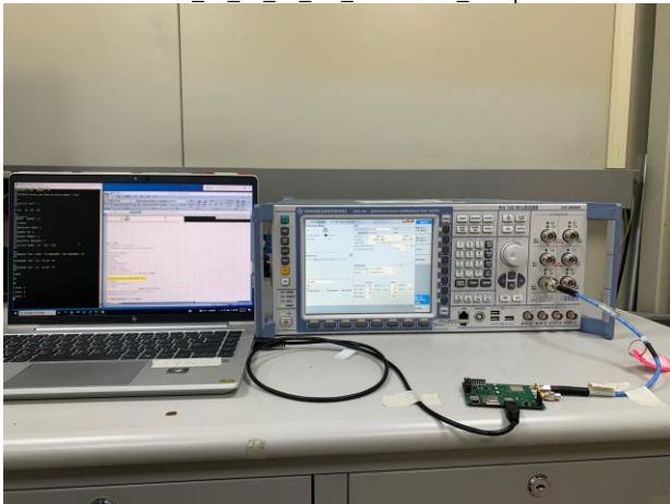
Part_22_24_27_NB-IOT_Conducted_Setup
