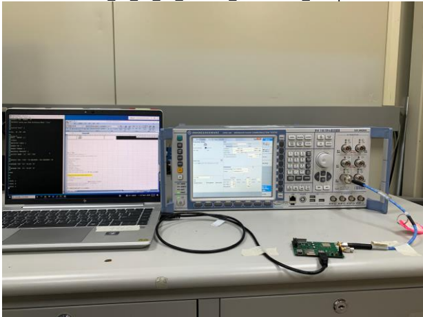
Part_25_Conducted_Setup
