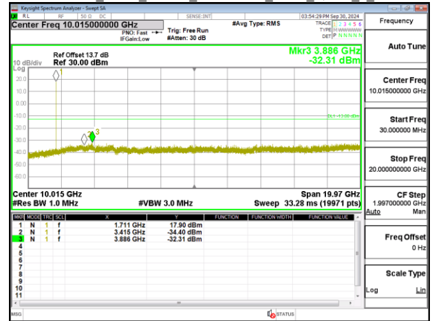
Band4 3MHz_Chain0 1732.5MHz_NBI 0 QPSK 1_0
