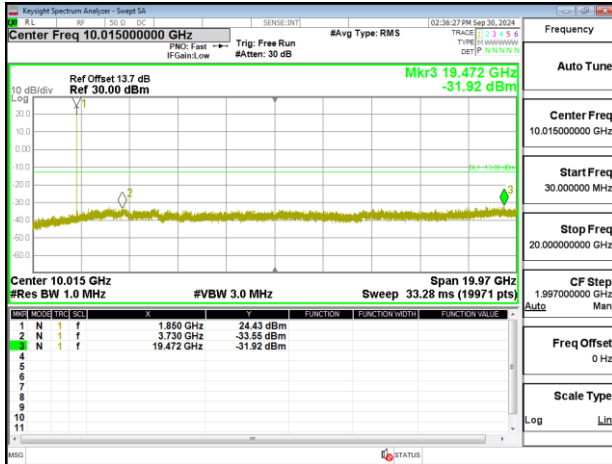
Band2_1.4MHz_Chain0_1880MHz_NBI_0_QPSK_1_0
