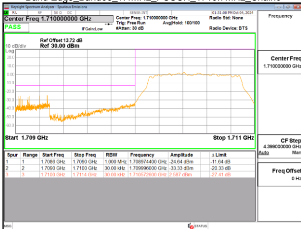
Band Edge_Band66_1.4MHz_PUSCH_1710.7MHz_Chain0
