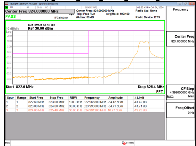
Band Edge_Band26_15MHz_PUSCH_831.5MHz_Chain0
