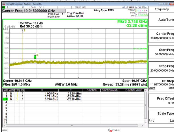
Band2_5MHz_Chain0_1907.5MHz_NBI_0_QPSK_1_0
