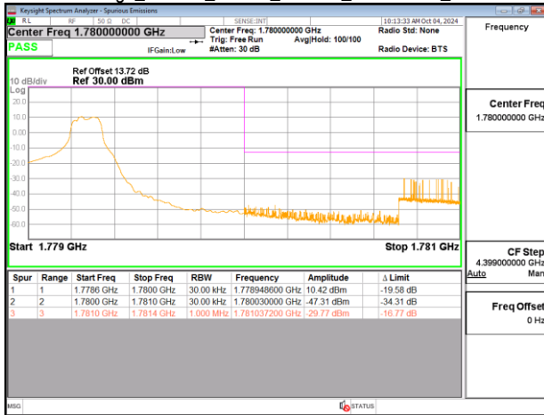
Band Edge_Band66_15MHz_PUSCH_1772.5MHz_Chain0
