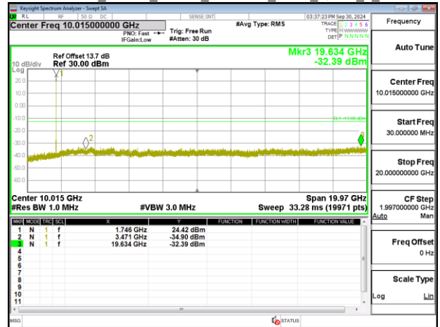
Band4_10MHz_Chain0_1750MHz_NBI_0_QPSK_1_0
