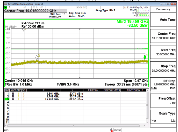
Band2_10MHz_Chain0_1905MHz_NBI_0_QPSK_1_0
