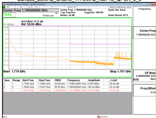
Band66_20MHz_Chain0_1770MHz_NBI 15_QPSK_6_0
