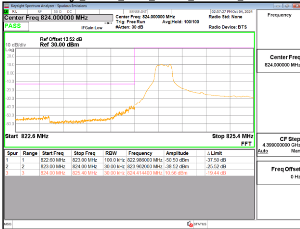
Band Edge_Band26_5MHz_PUSCH_826.5MHz_Chain0
