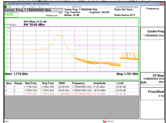
Band Edge_Band66_5MHz_PUSCH_1777.5MHz_Chain0
