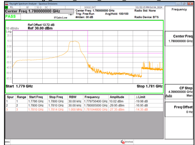
Band Edge_Band66_1.4MHz_PUSCH_1779.3MHz_Chain0
