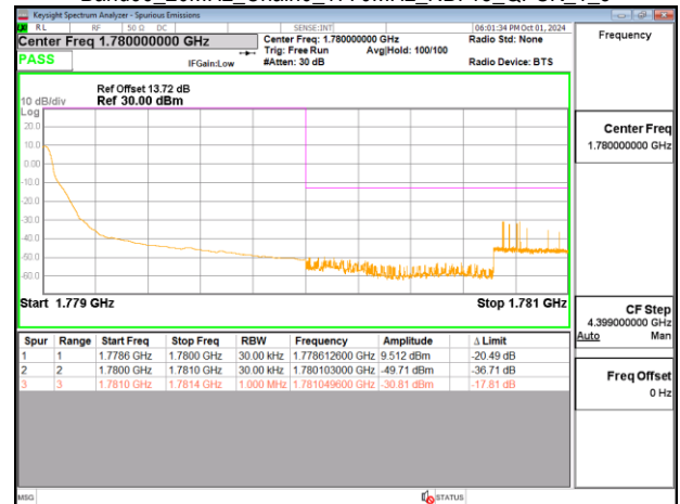
Band66_20MHz_Chain0_1770MHz_NBI 15_QPSK_1 5
