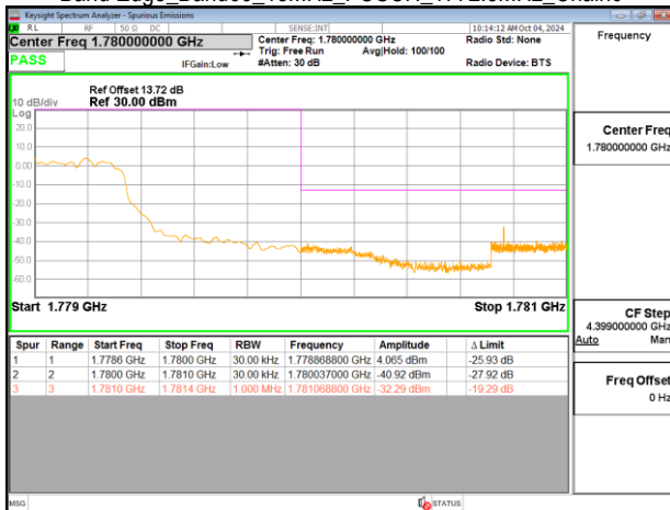
Band Edge_Band66_15MHz_PUSCH_1772.5MHz_Chain0
