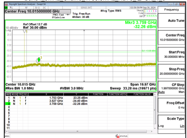
Band4 3MHz_Chain0 1753.5MHz_NBI 0 QPSK 1_0
