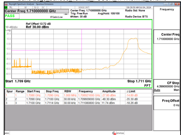
Band Edge_Band66_15MHz_PUSCH_1717.5MHz_Chain0
