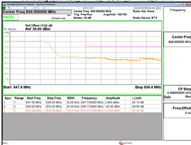
Band Edge_Band26_10MHz_PUSCH_844MHz_Chain0
