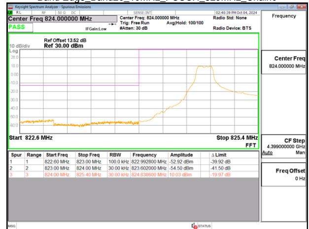
Band Edge_Band26_10MHz_PUSCH_829MHz_Chain0
