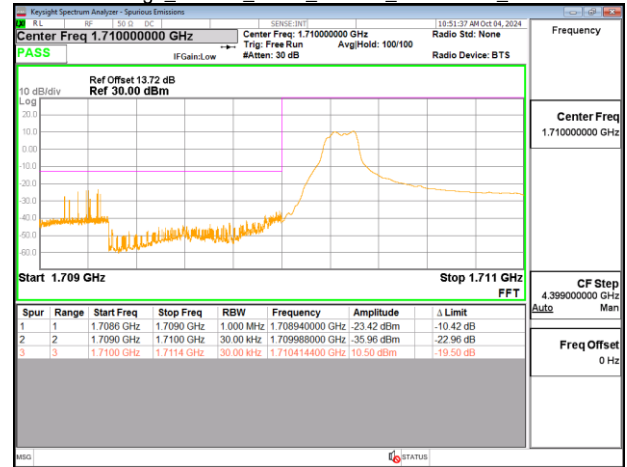
Band Edge_Band66_5MHz_PUSCH_1712.5MHz_Chain0
