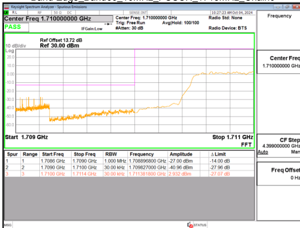
Band Edge_Band66_10MHz_PUSCH_1715MHz_Chain0
