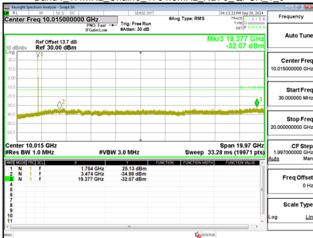
Band4 1.4MHz_Chain0 1754.3MHz_NBI 0 QPSK 1_0
