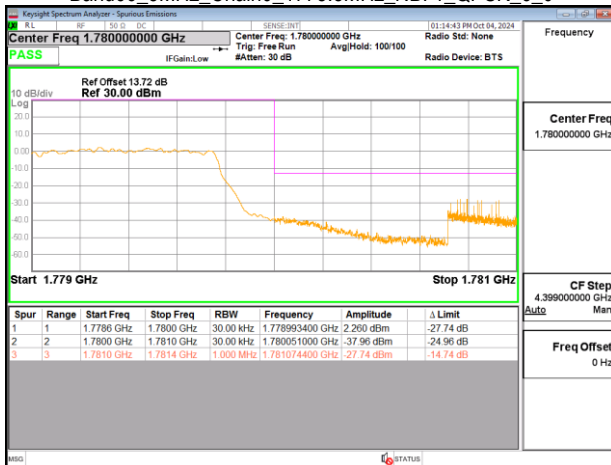
Band66_3MHz_Chain0_1778.5MHz_NBI 1_QPSK_6 0
