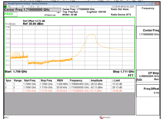
Band66_3MHz_Chain0_1711.5MHz_NBI_0_QPSK_1_0
