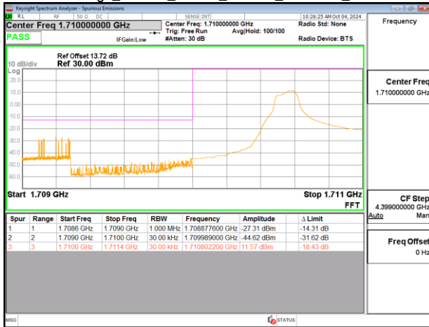
Band Edge_Band66_10MHz_PUSCH_1715MHz_Chain0
