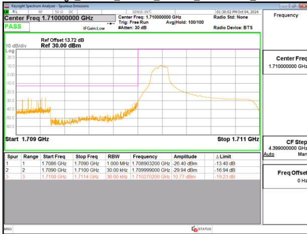
Band Edge_Band66_1.4MHz_PUSCH_1710.7MHz_Chain0
