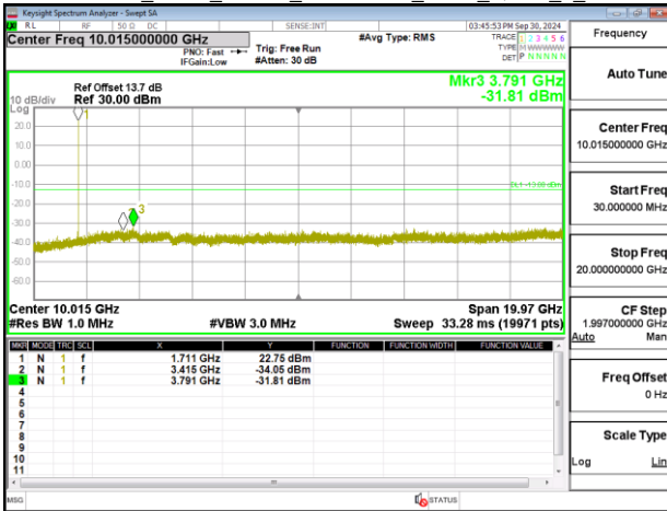
Band4_5MHz_Chain0_1732.5MHz_NBI_0_QPSK_1_0
