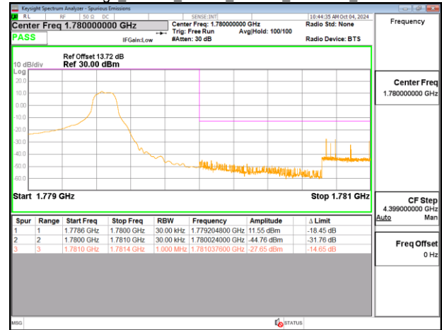
Band Edge_Band66_10MHz_PUSCH_1775MHz_Chain0
