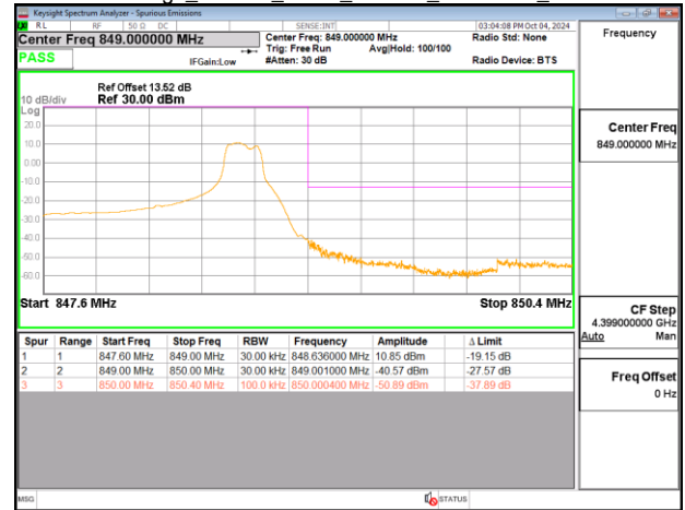
Band Edge_Band26_5MHz_PUSCH_846.5MHz_Chain0
