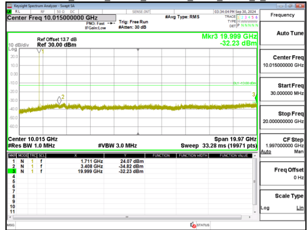
Band4_10MHz_Chain0_1732.5MHz_NBI_0_QPSK_1_0
