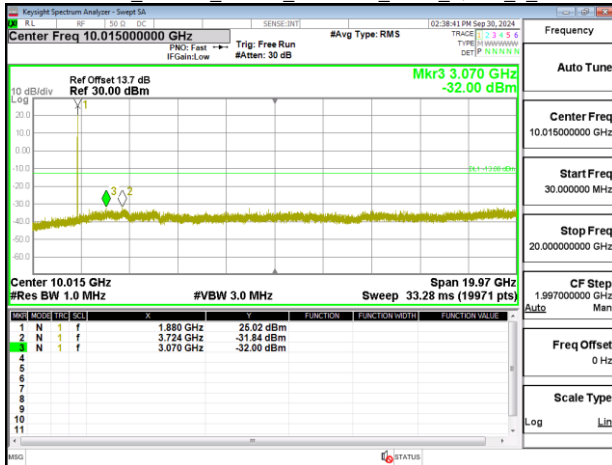
Band2_1.4MHz_Chain0_1909.3MHz_NBI_0_QPSK_1_0
