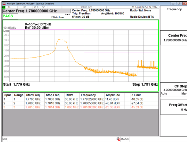
Band66_3MHz_Chain0_1778.5MHz_NBI 1_QPSK_6 0
