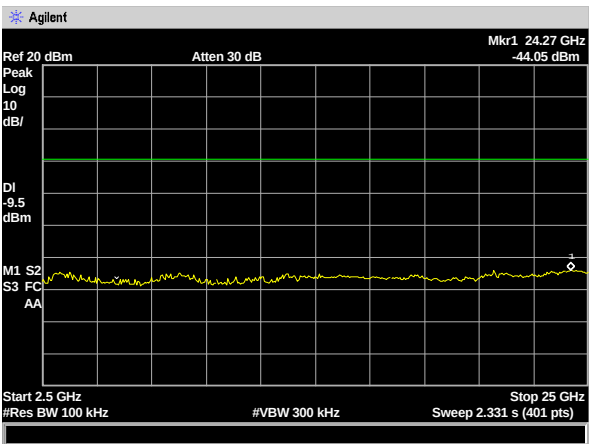
Figure 7.6.2.2-6: 2.5 GHz – 25 GHz –High Channel
