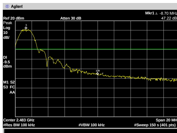
Figure 7.6.1.2-2: Upper Band-edge (Conducted)
