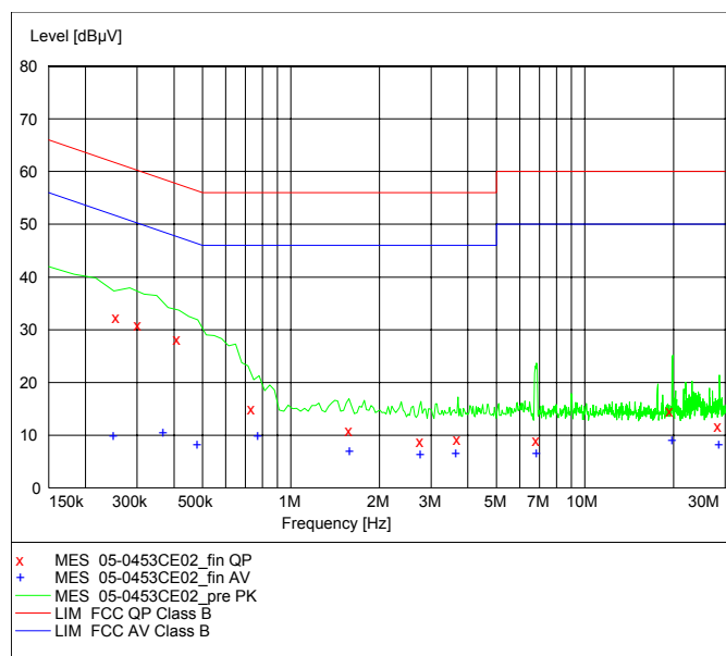
Figure 7.2-2: Conducted Emissions Graph – Line 2
