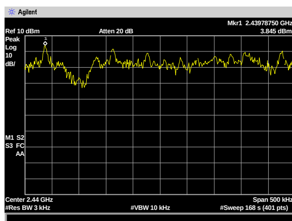
Figure 7.7.2-2: Power Spectral Density Plot – Mid Channel
